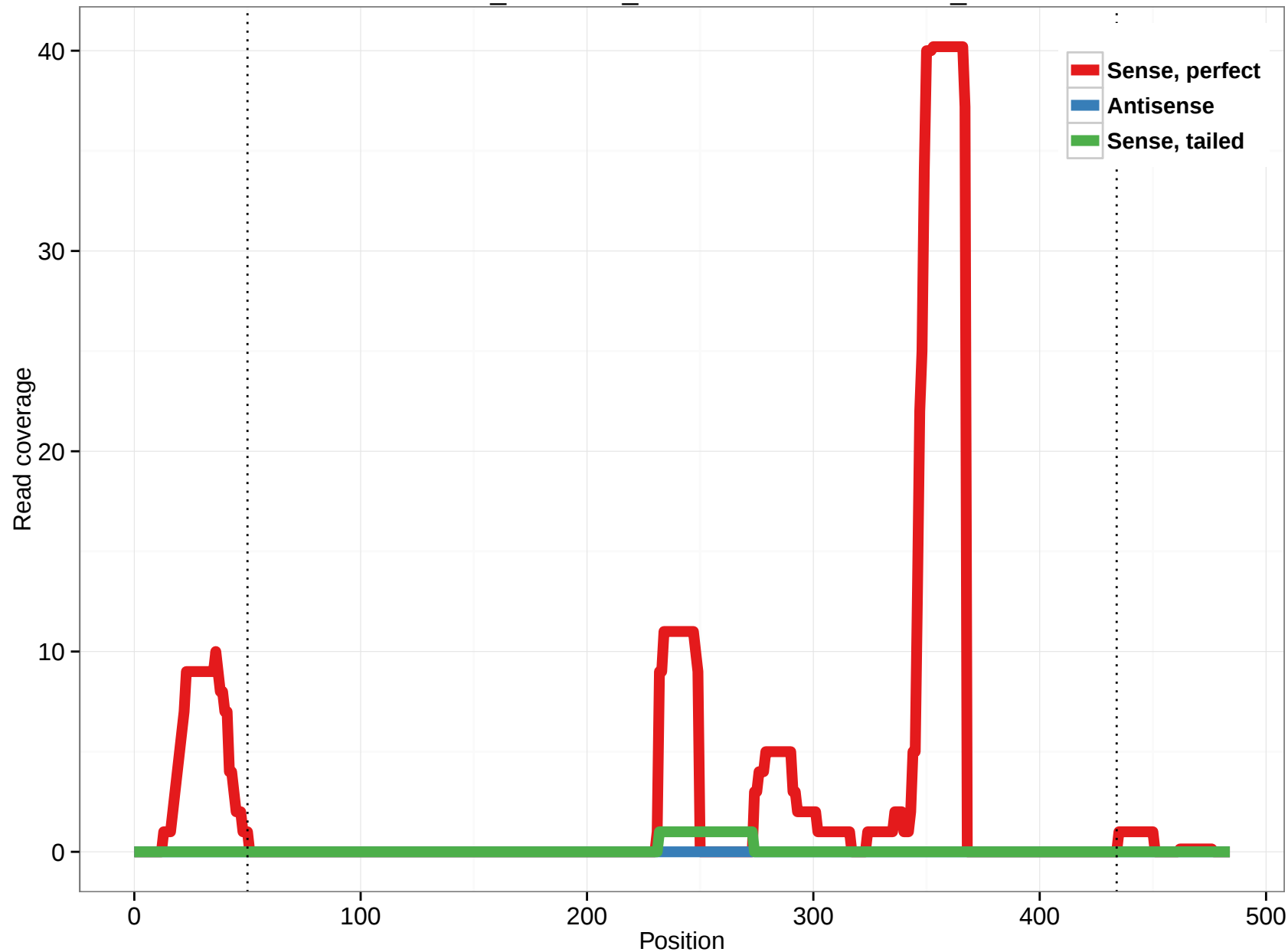
ornAna1_ensGene_ENSOANT00000017452_4
