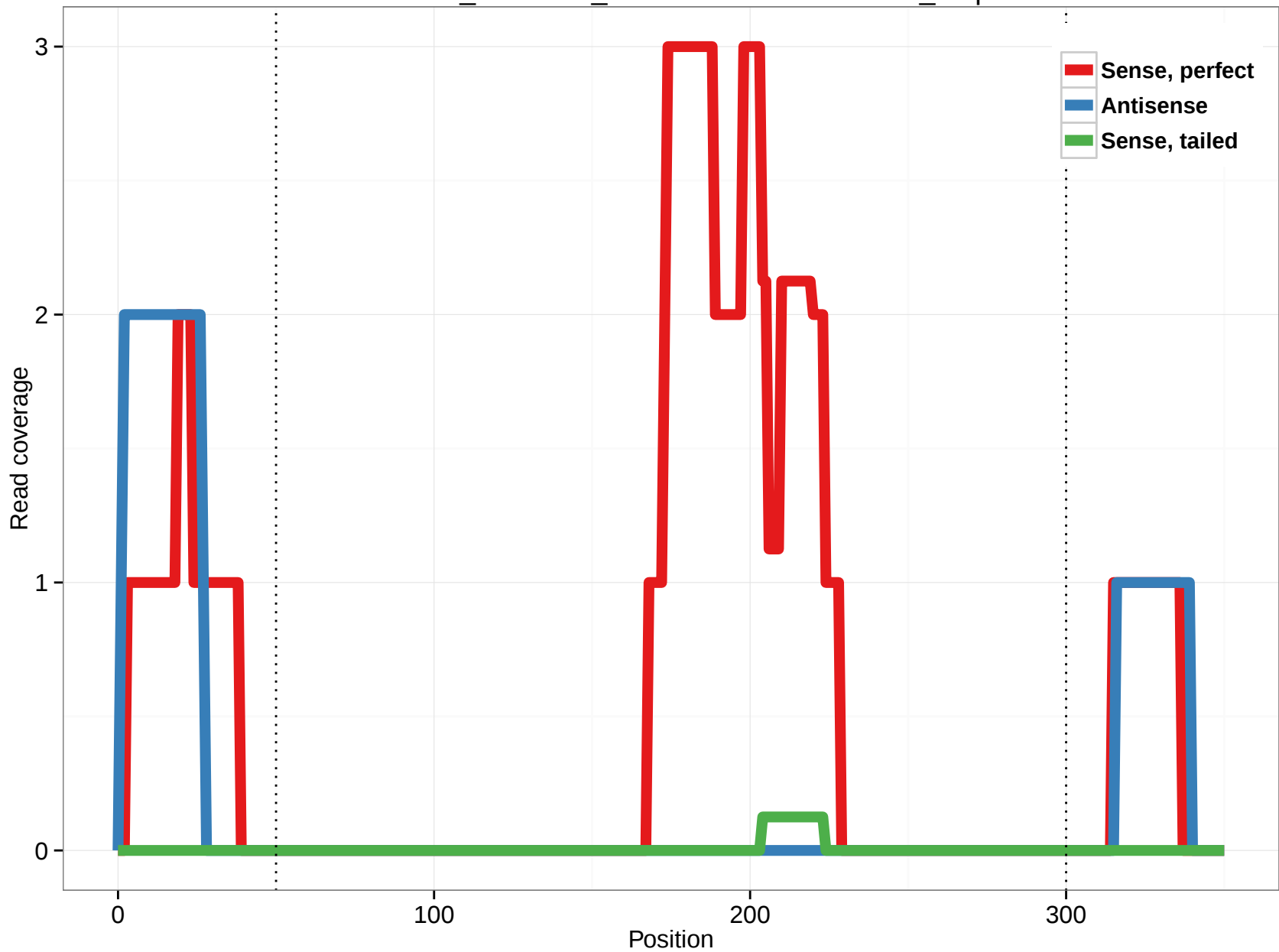
ornAna1_ensGene_ENSOANT00000017245_5.5p
