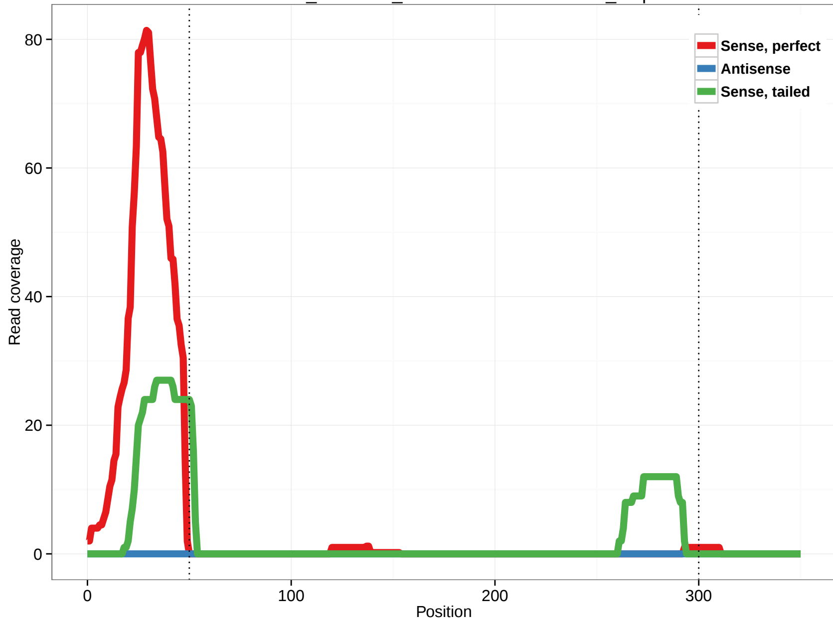
ornAna1_ensGene_ENSOANT00000017230_0.5p
