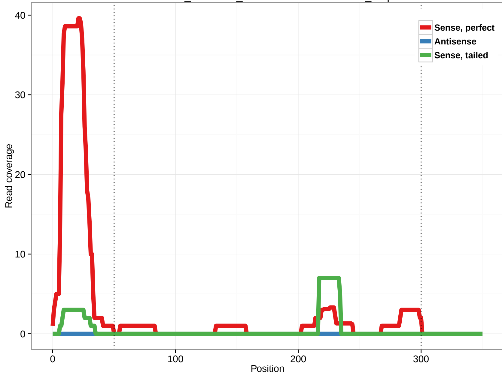
ornAna1_ensGene_ENSOANT00000017226_1.5p
