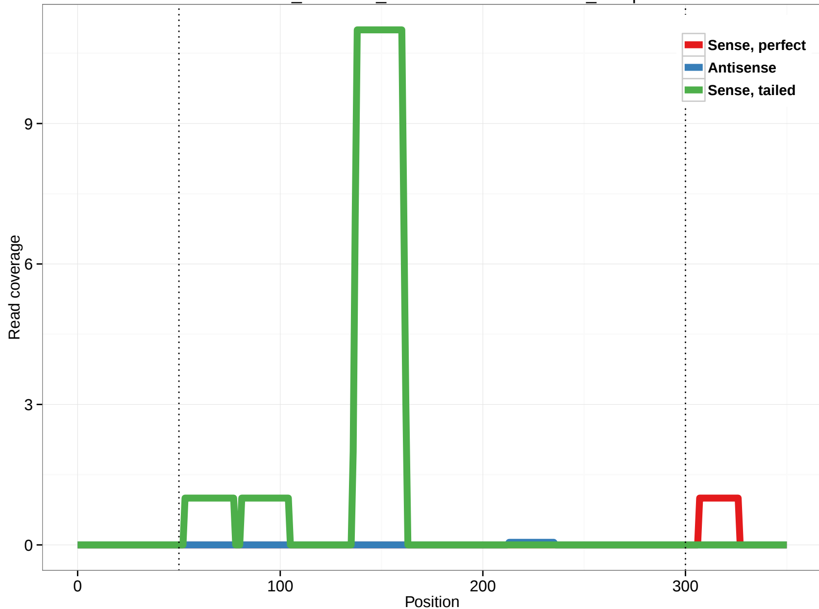
ornAna1_ensGene_ENSOANT00000017224_11.3p
