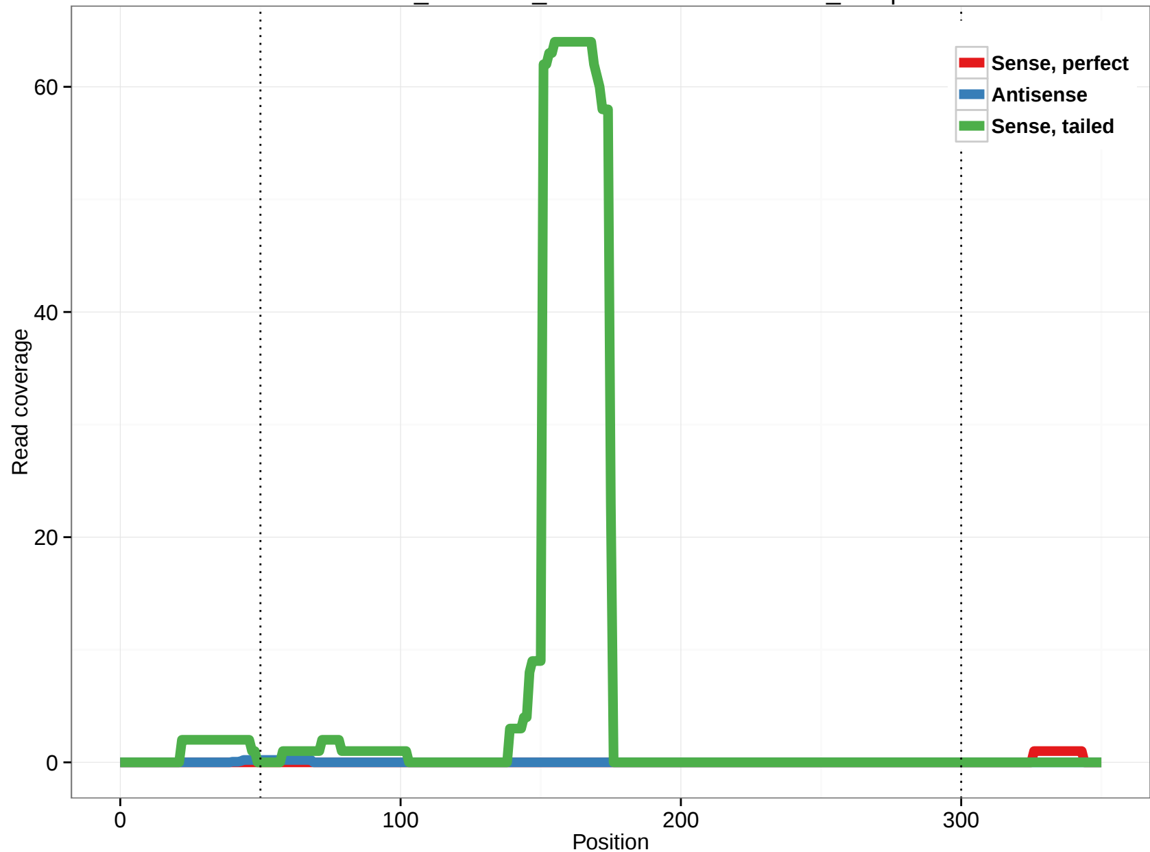
ornAna1_ensGene_ENSOANT00000017180_10.3p
