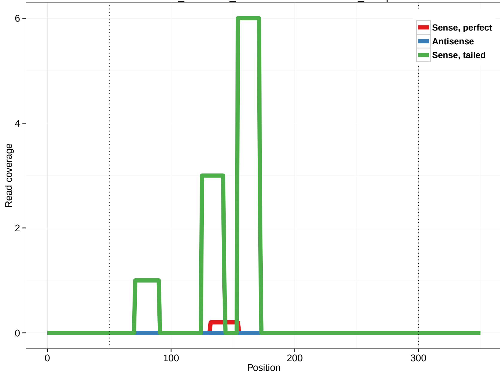
ornAna1_ensGene_ENSOANT00000017132_17.3p
