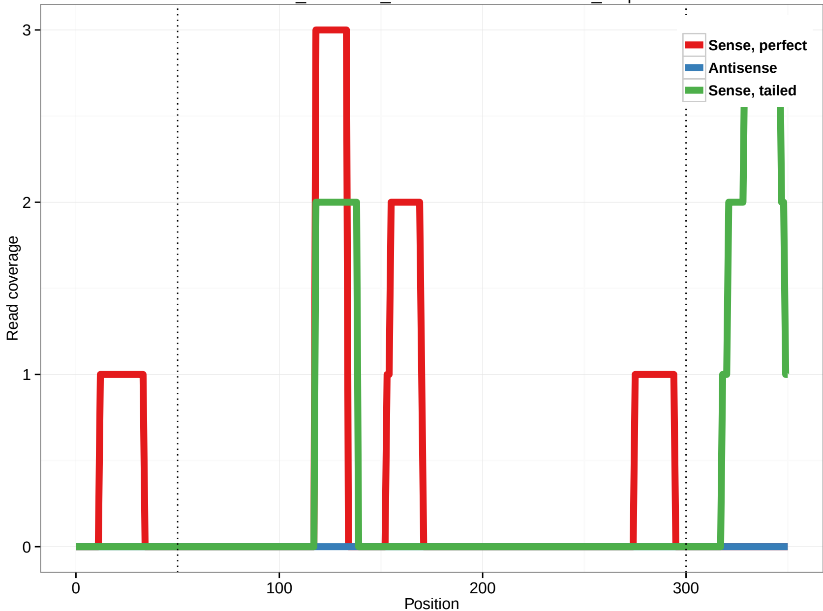
ornAna1_ensGene_ENSOANT00000017129_8.5p
