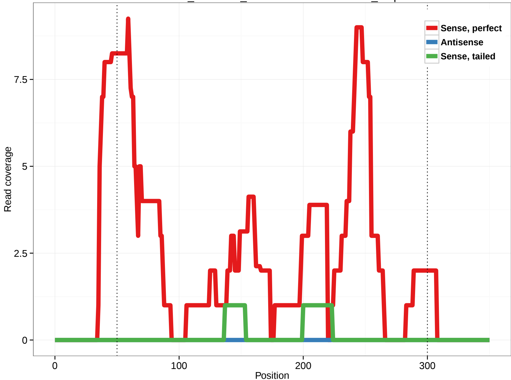
ornAna1_ensGene_ENSOANT00000016980_2.5p
