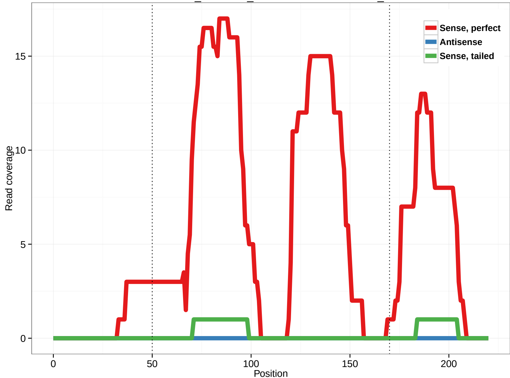
ornAna1_ensGene_ENSOANT00000016980_1
