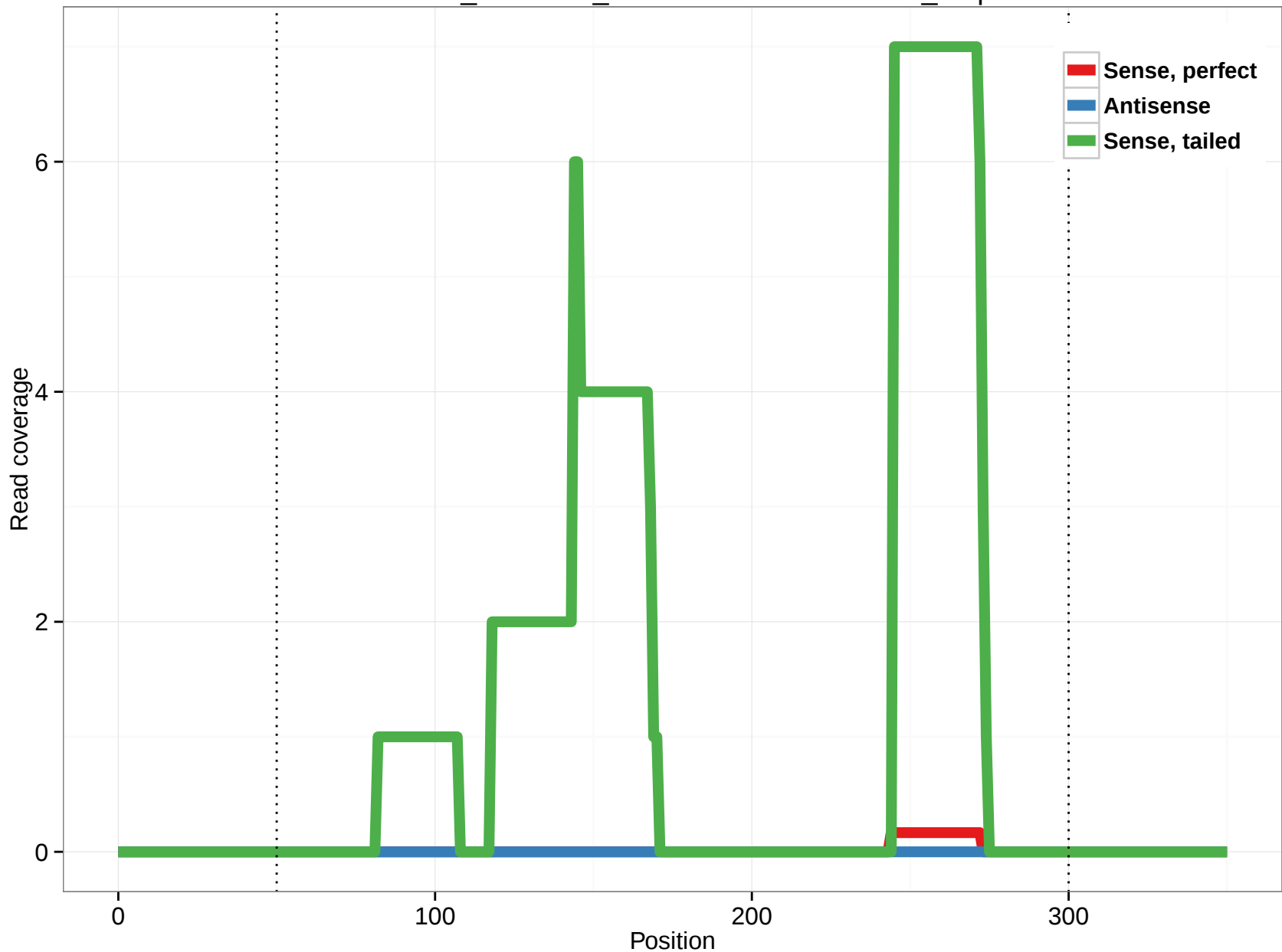
ornAna1_ensGene_ENSOANT00000016953_3.5p
