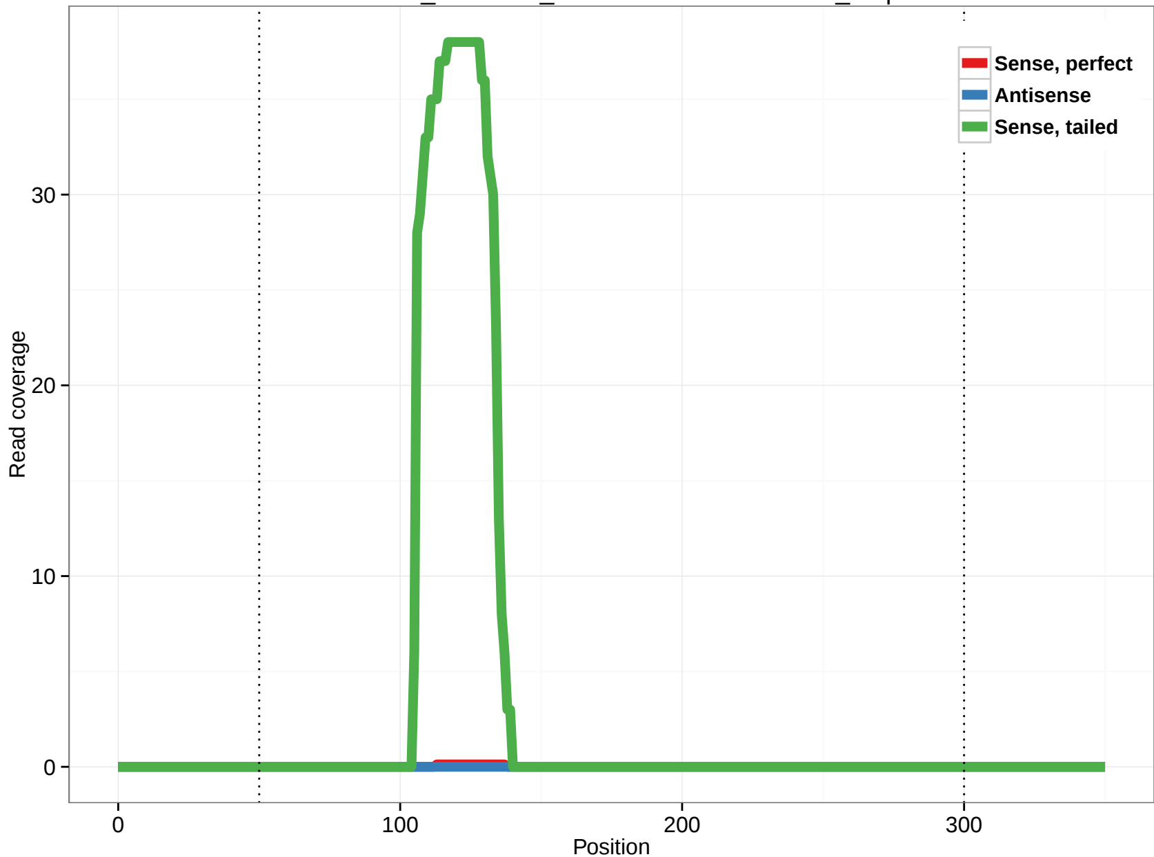
ornAna1_ensGene_ENSOANT00000016933_2.3p
