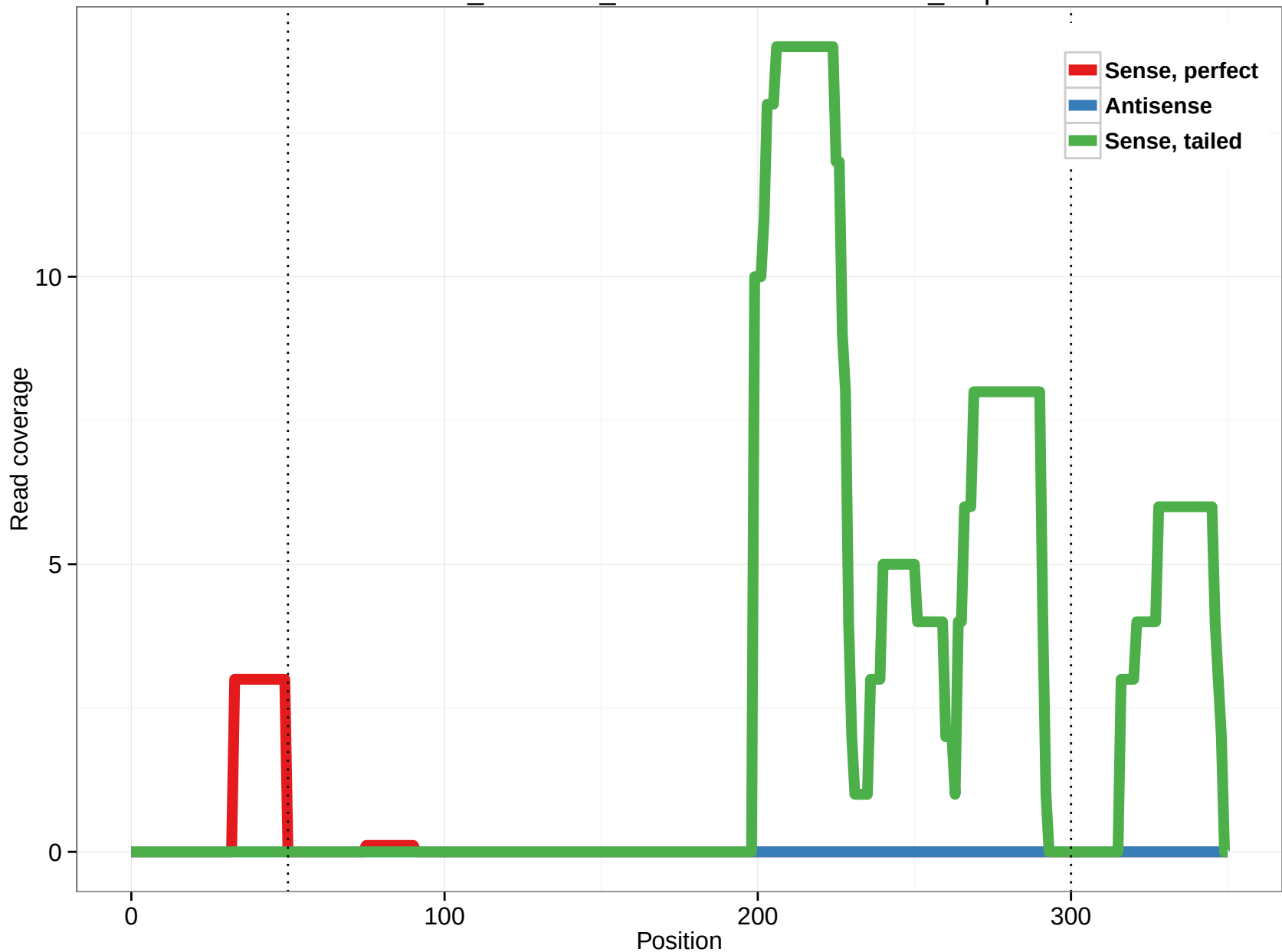
ornAna1_ensGene_ENSOANT00000016926_2.5p
