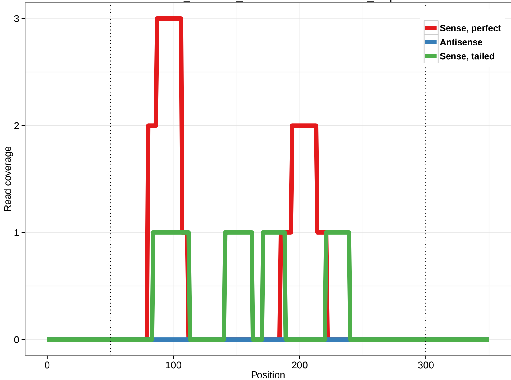
ornAna1_ensGene_ENSOANT00000016894_7.5p
