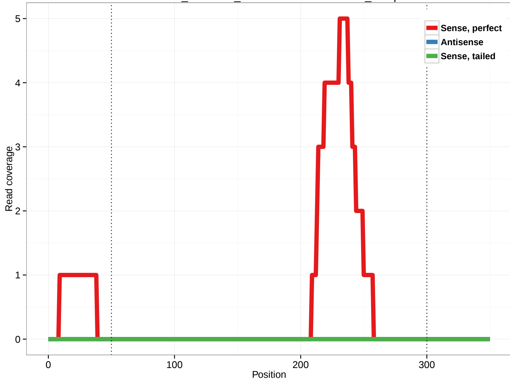
ornAna1_ensGene_ENSOANT00000016893_11.5p
