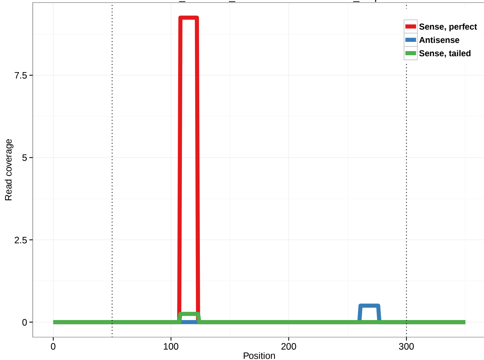
ornAna1_ensGene_ENSOANT00000016885_0.3p
