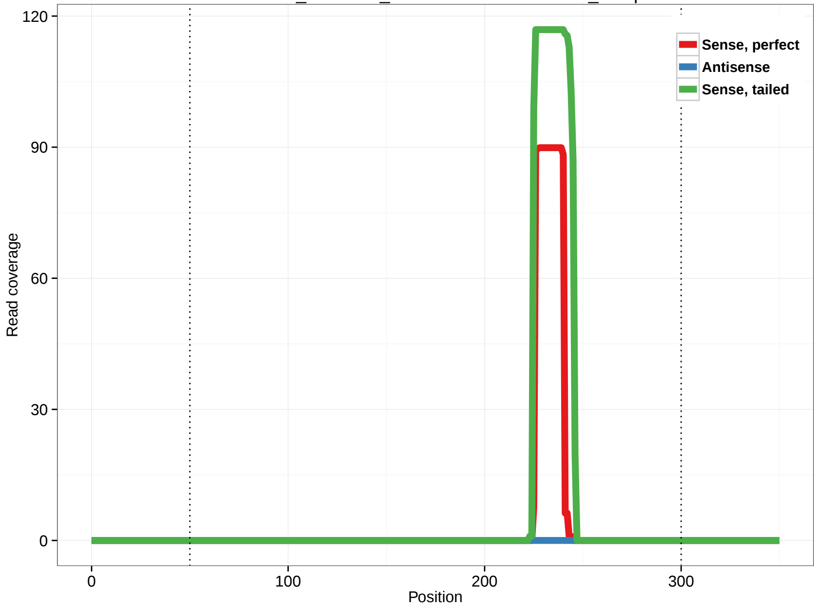
ornAna1_ensGene_ENSOANT00000016844_26.5p
