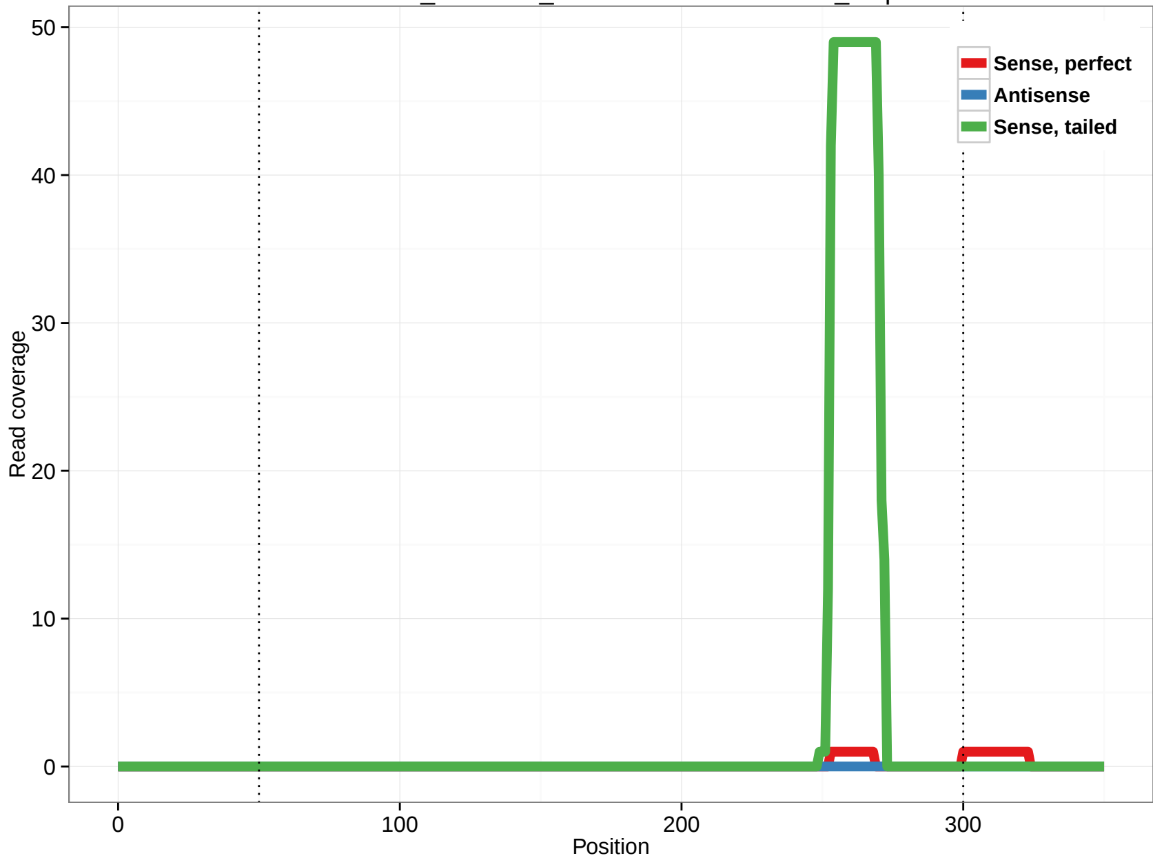
ornAna1_ensGene_ENSOANT00000016838_4.3p
