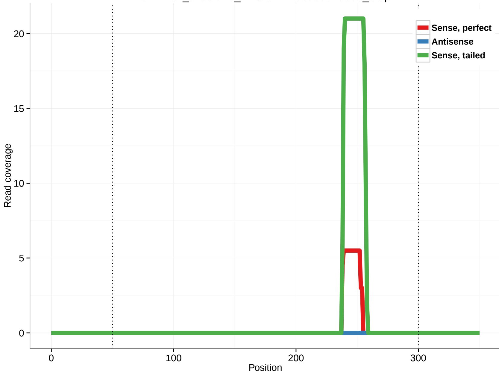
ornAna1_ensGene_ENSOANT00000016805_6.5p
