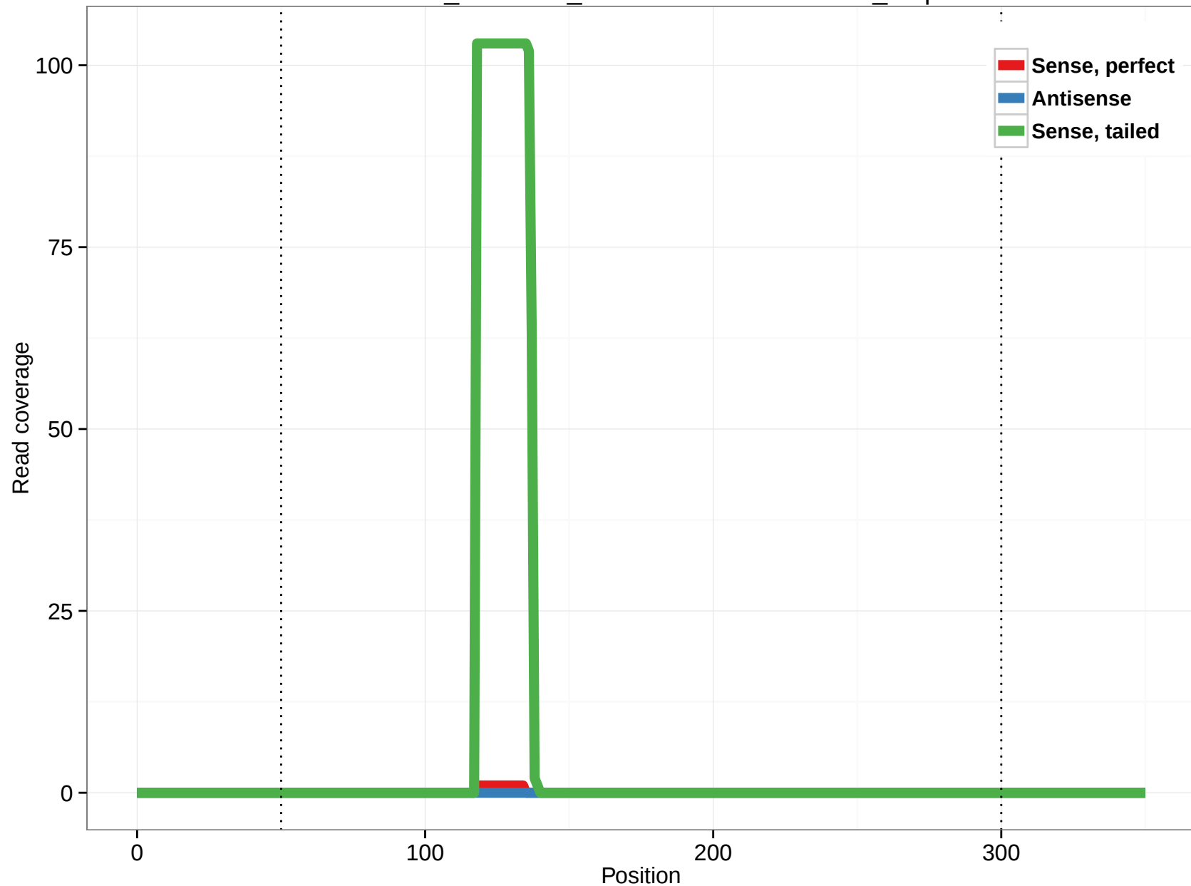
ornAna1_ensGene_ENSOANT00000016768_4.3p
