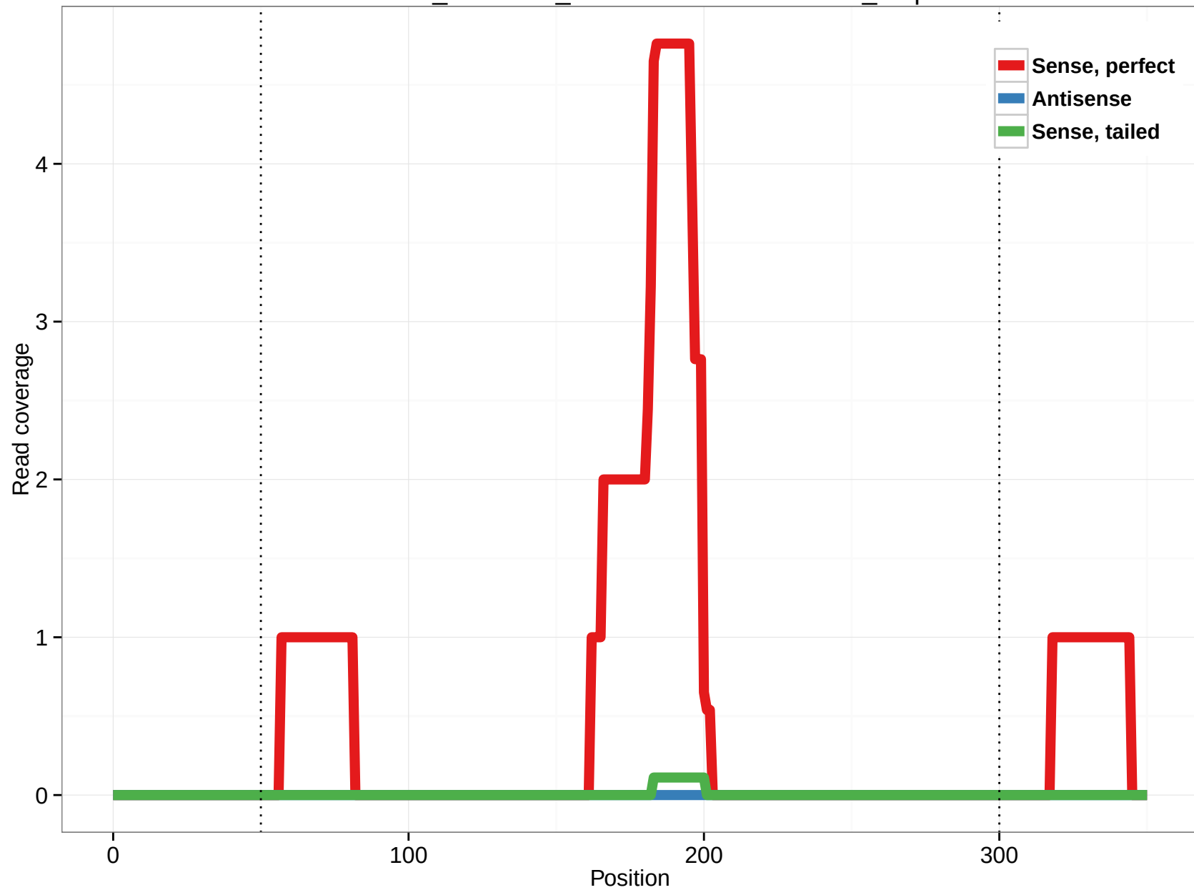
ornAna1_ensGene_ENSOANT00000016728_0.3p
