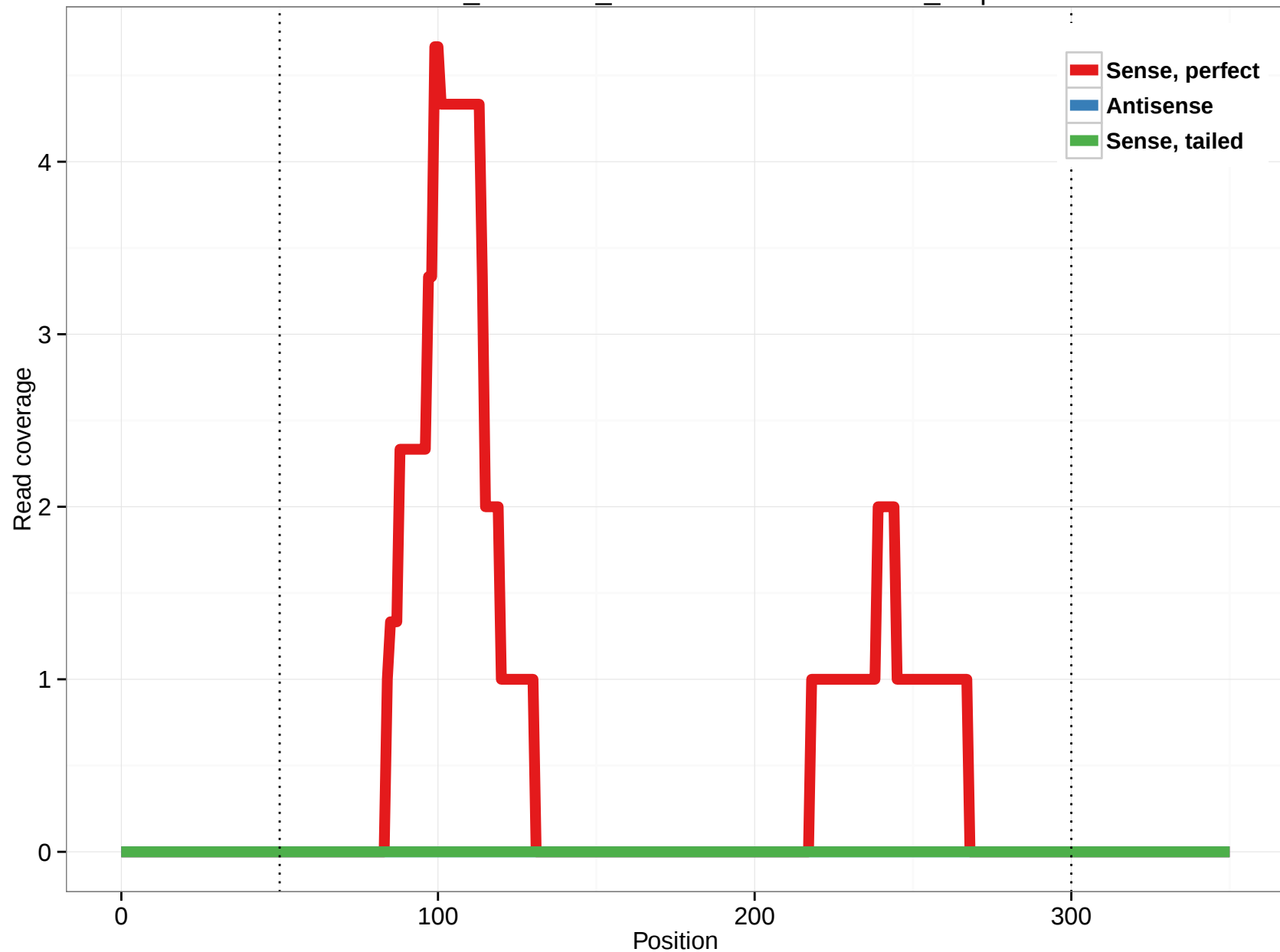
ornAna1_ensGene_ENSOANT00000016504_2.5p
