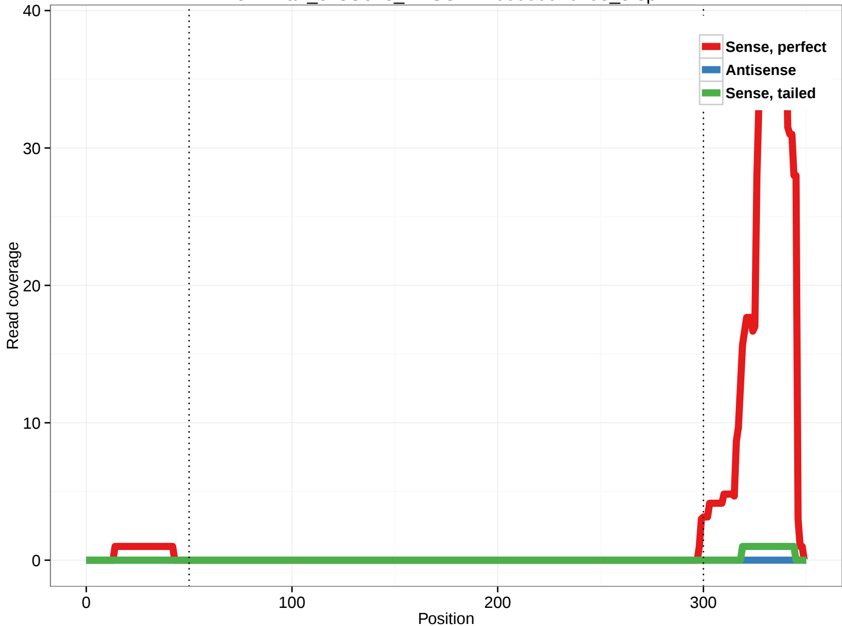
ornAna1_ensGene_ENSOANT00000016493_5.3p
