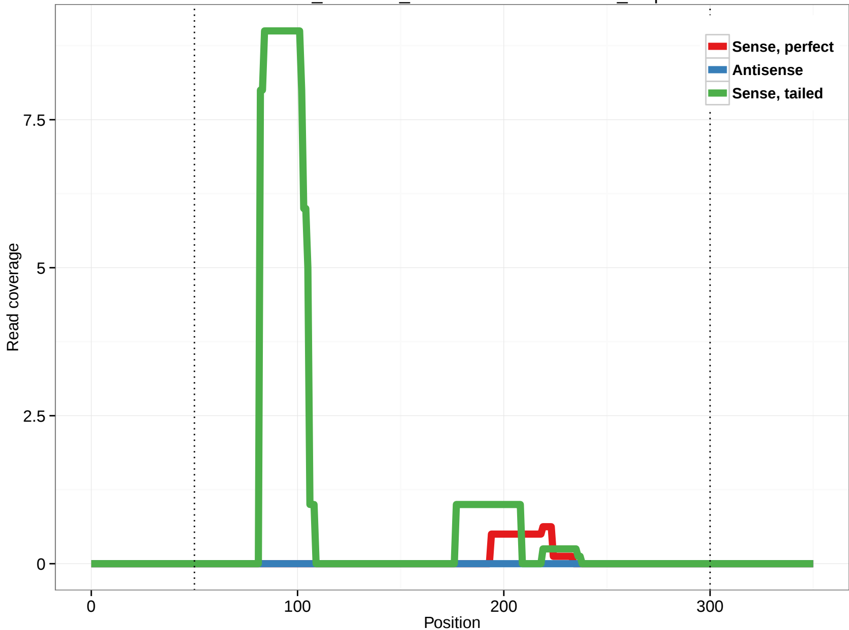
ornAna1_ensGene_ENSOANT00000016397_1.3p
