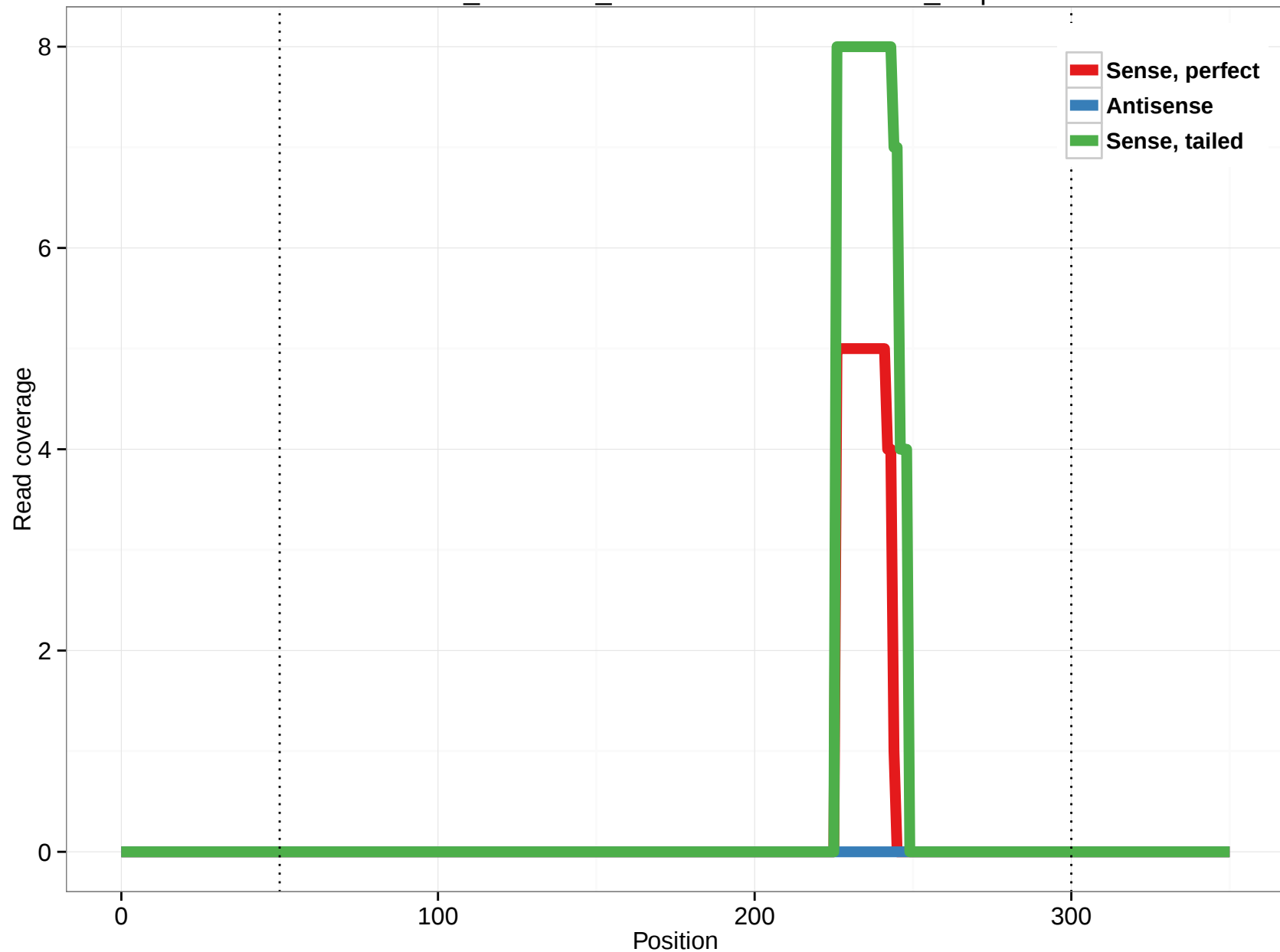
ornAna1_ensGene_ENSOANT00000016362_2.3p
