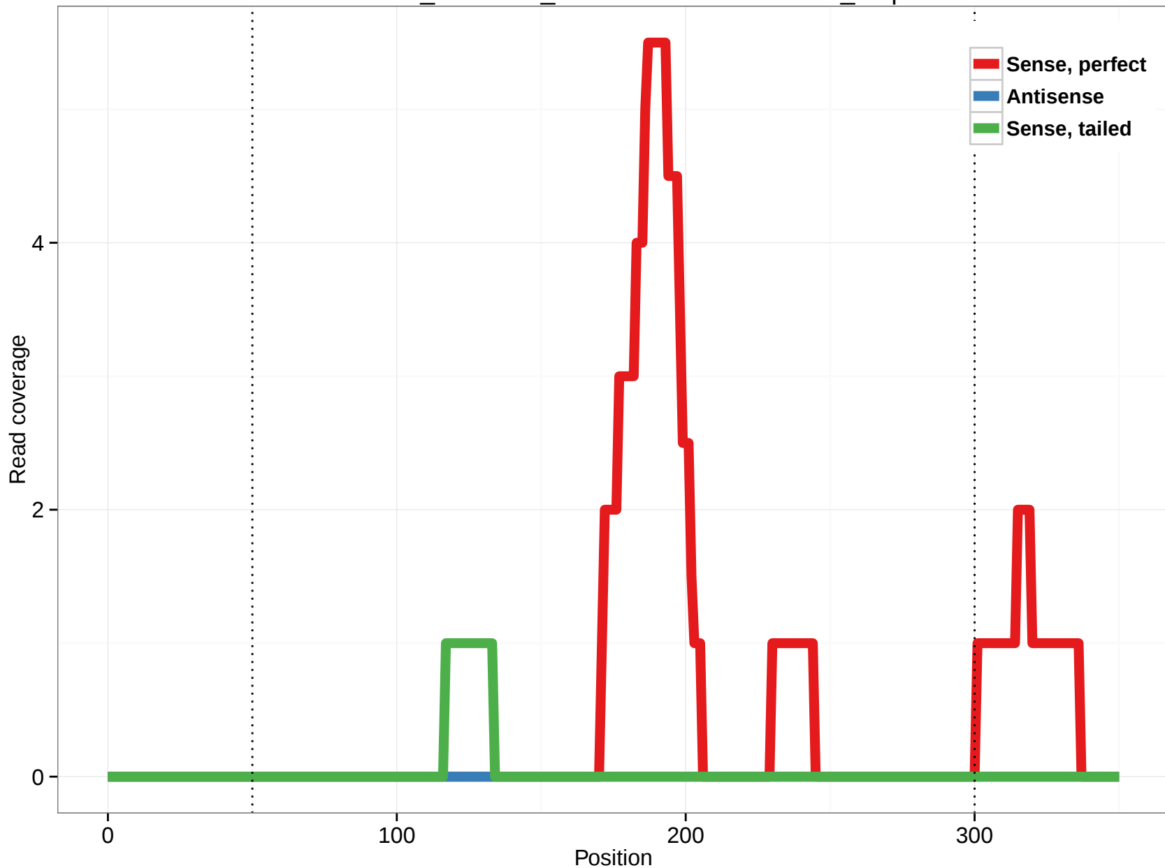
ornAna1_ensGene_ENSOANT00000016320_1.3p
