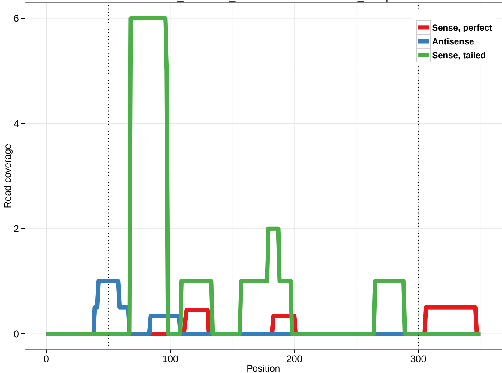
ornAna1_ensGene_ENSOANT00000016318_73.3p
