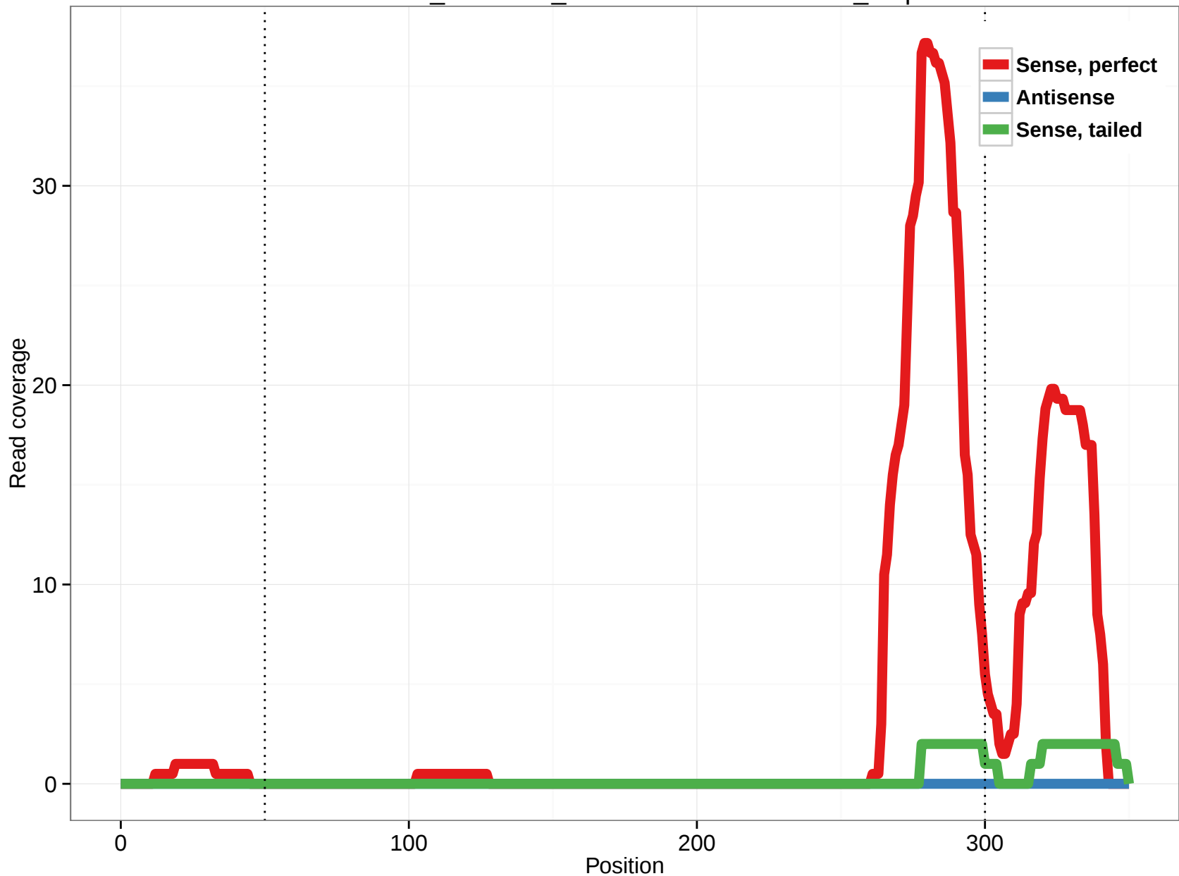
ornAna1_ensGene_ENSOANT00000016297_1.3p
