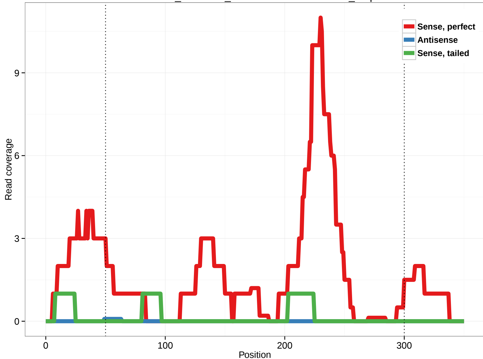
ornAna1_ensGene_ENSOANT00000016239_1.3p
