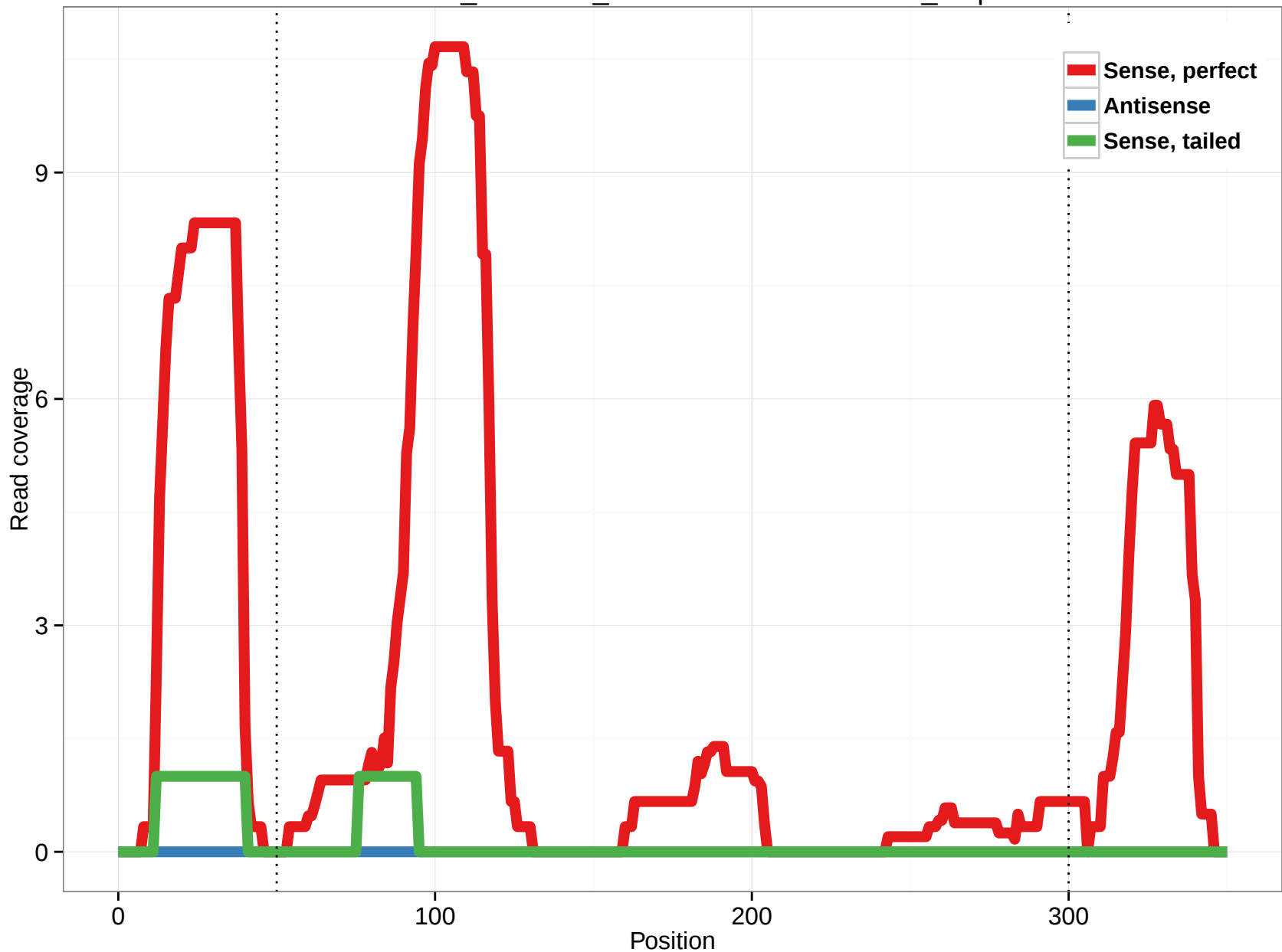
ornAna1_ensGene_ENSOANT00000016229_0.3p
