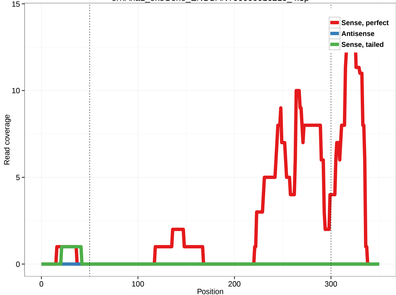
ornAna1_ensGene_ENSOANT00000016210_4.3p
