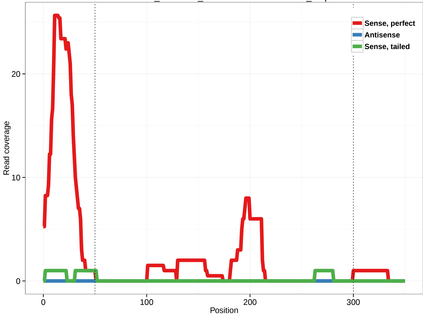
ornAna1_ensGene_ENSOANT00000016210_3.5p
