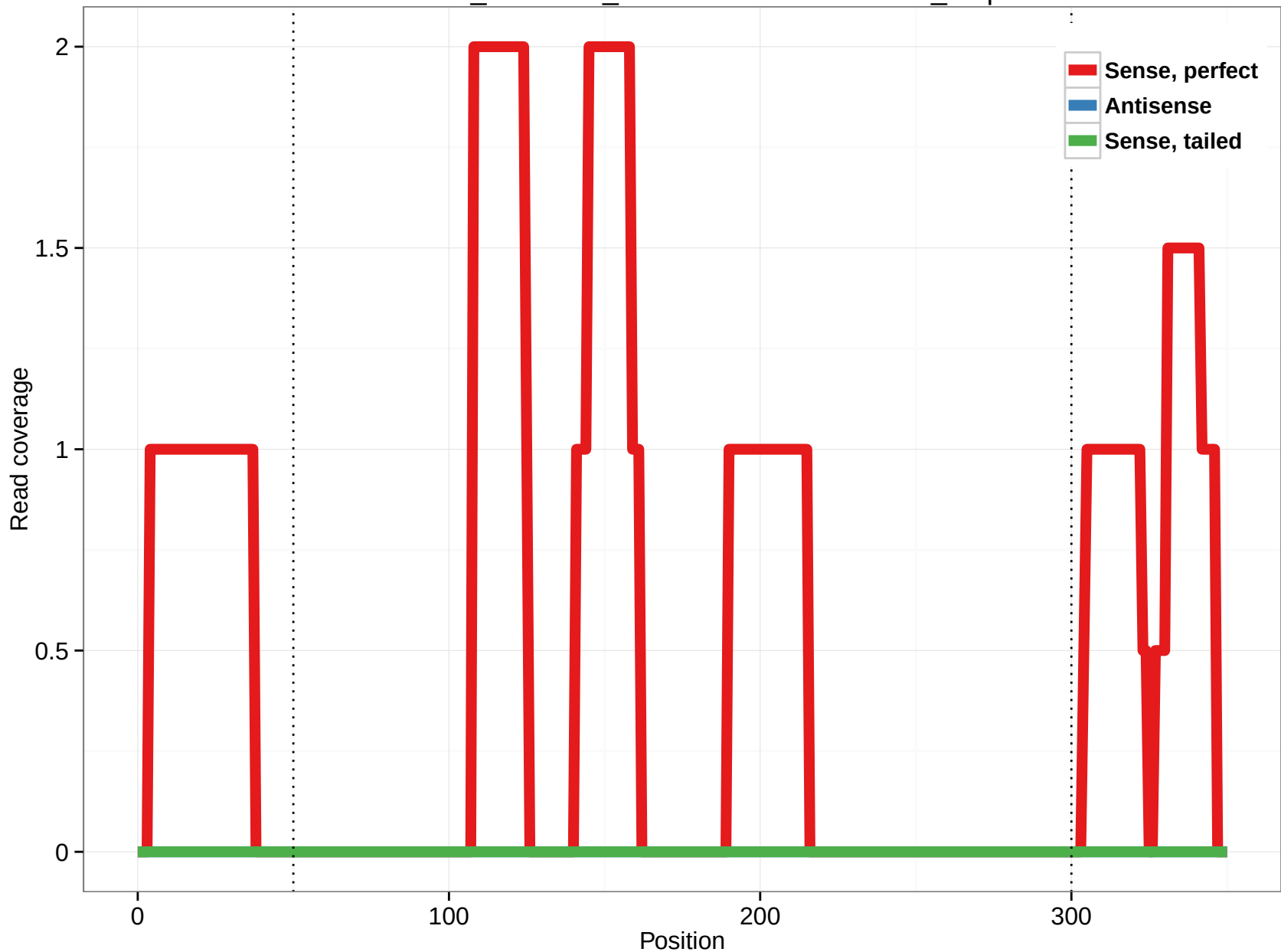
ornAna1_ensGene_ENSOANT00000016210_3.3p
