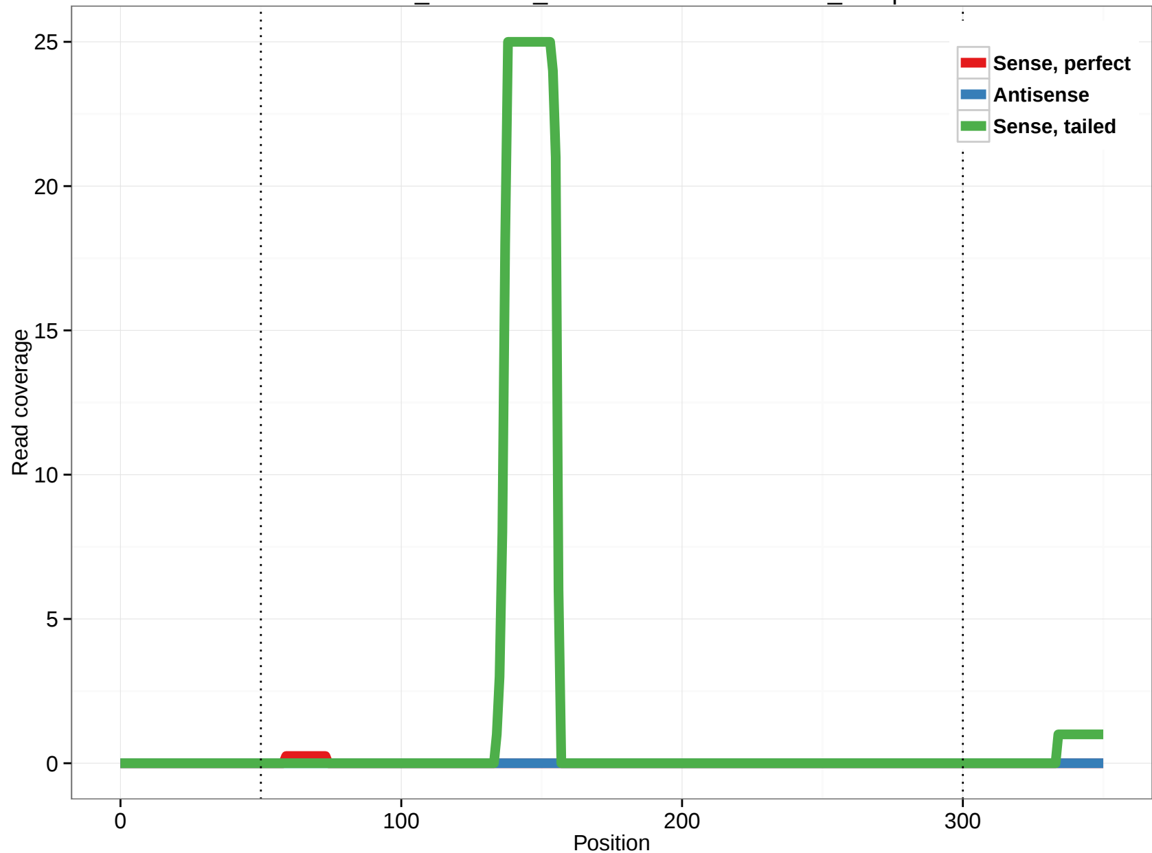
ornAna1_ensGene_ENSOANT00000016193_10.5p
