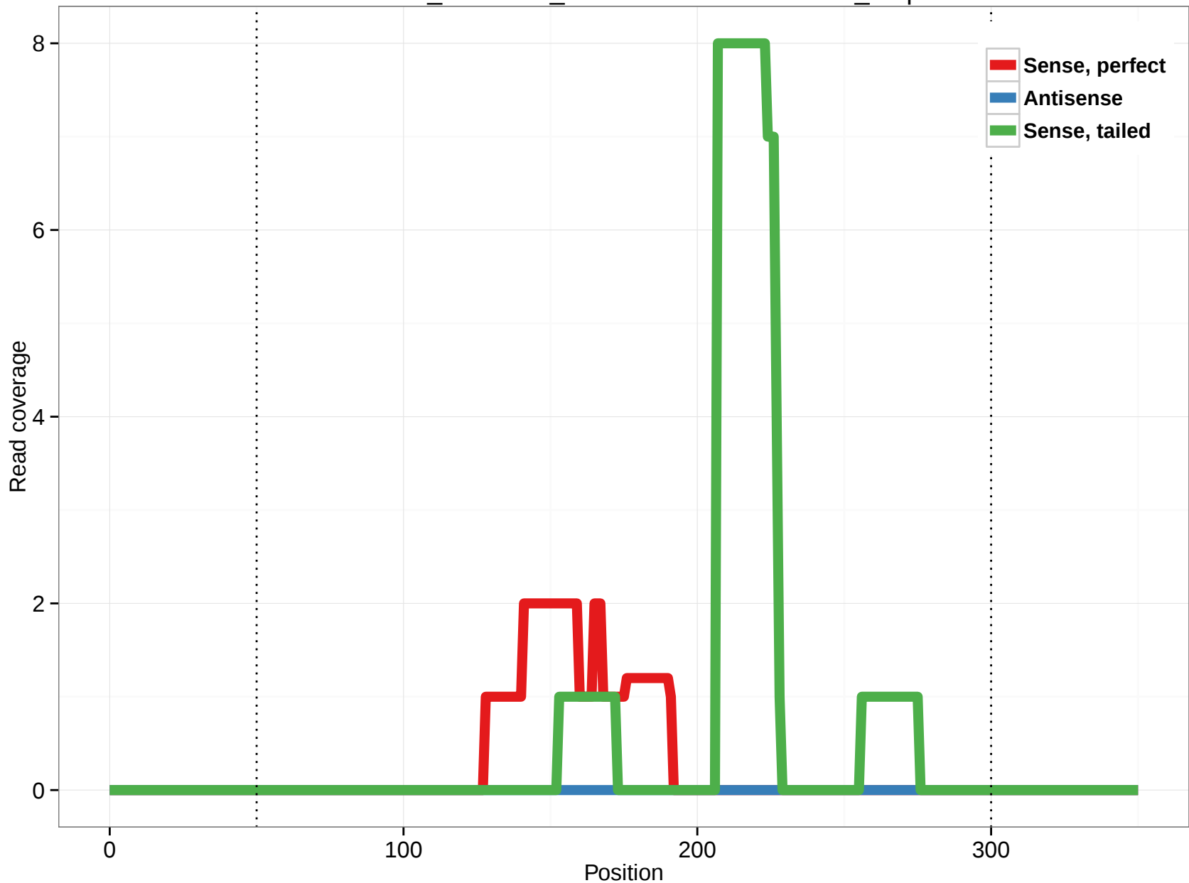
ornAna1_ensGene_ENSOANT00000016143_1.5p
