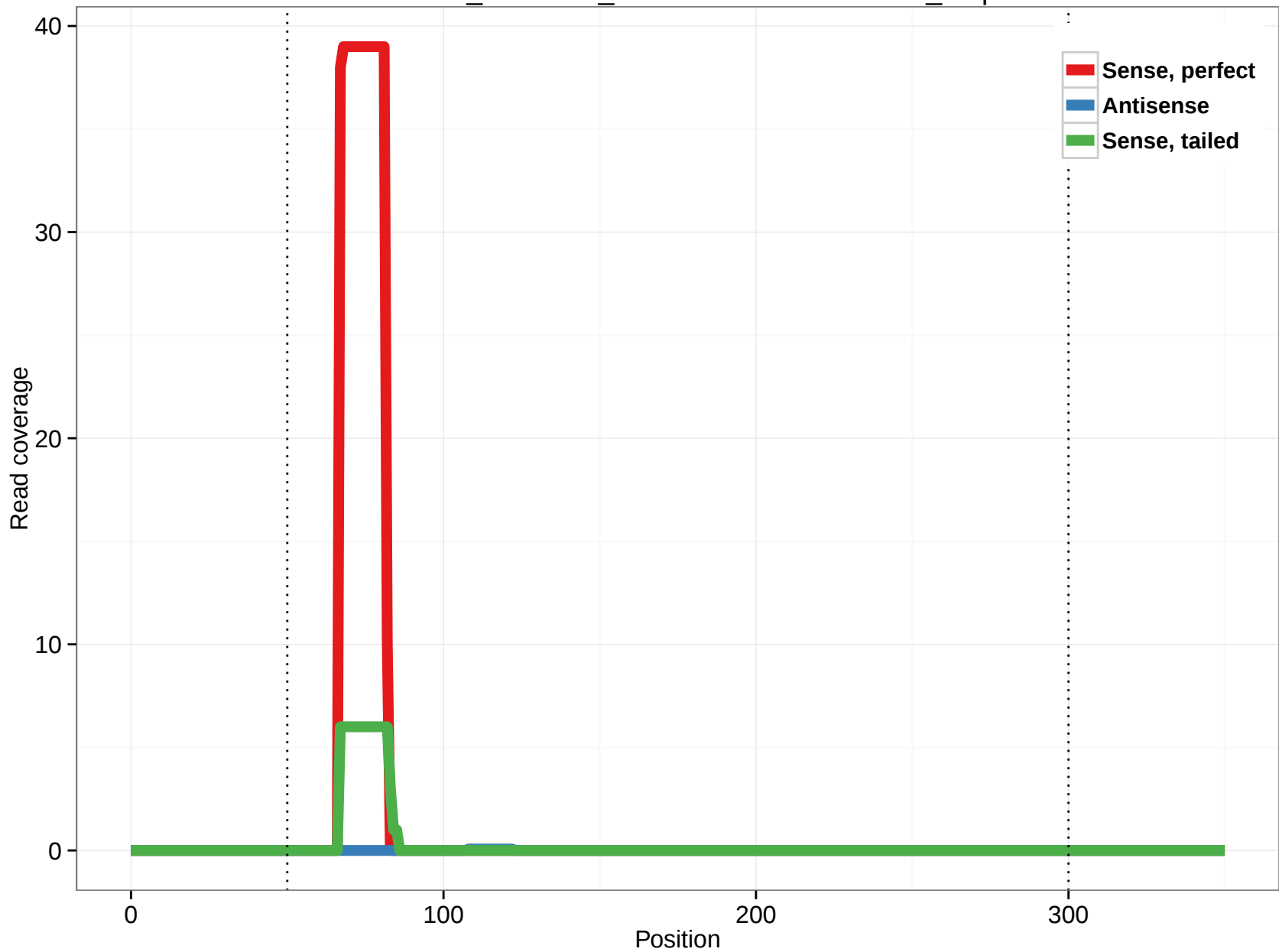
ornAna1_ensGene_ENSOANT00000016111_9.5p
