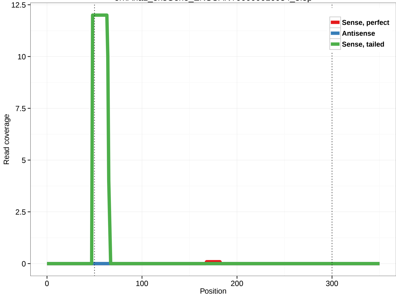
ornAna1_ensGene_ENSOANT00000016034_8.5p
