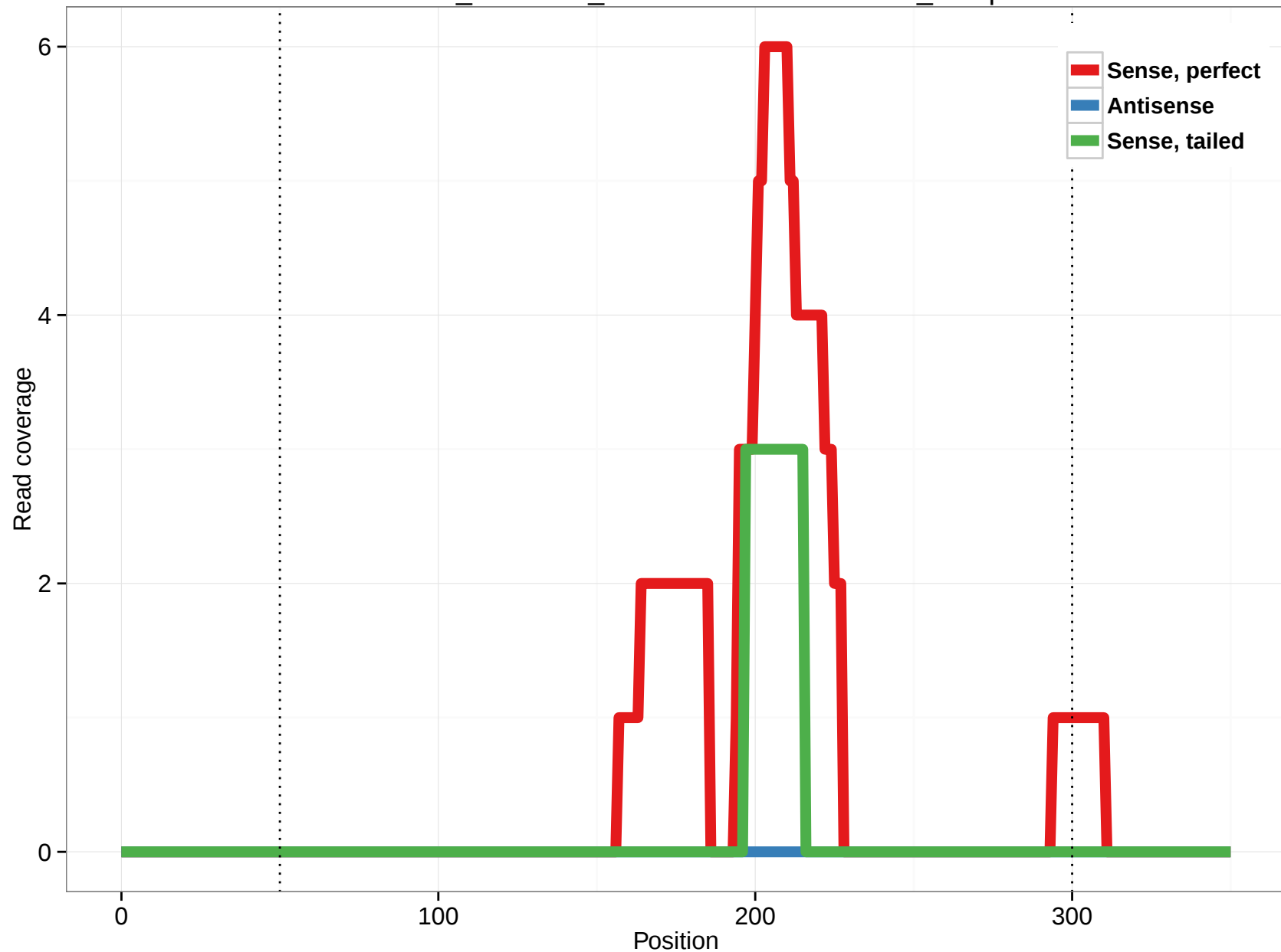
ornAna1_ensGene_ENSOANT00000016007_10.5p
