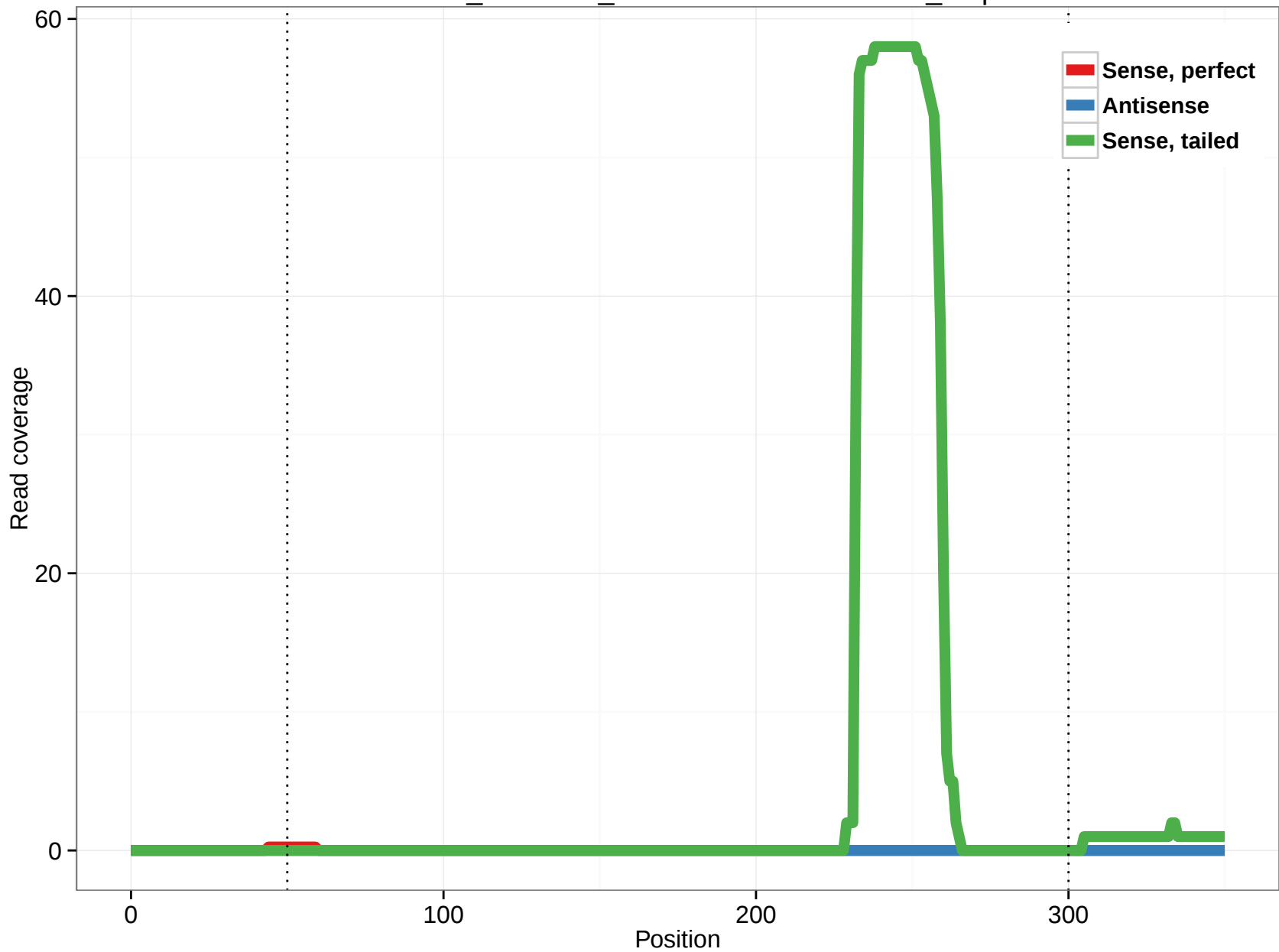
ornAna1_ensGene_ENSOANT00000015990_7.3p
