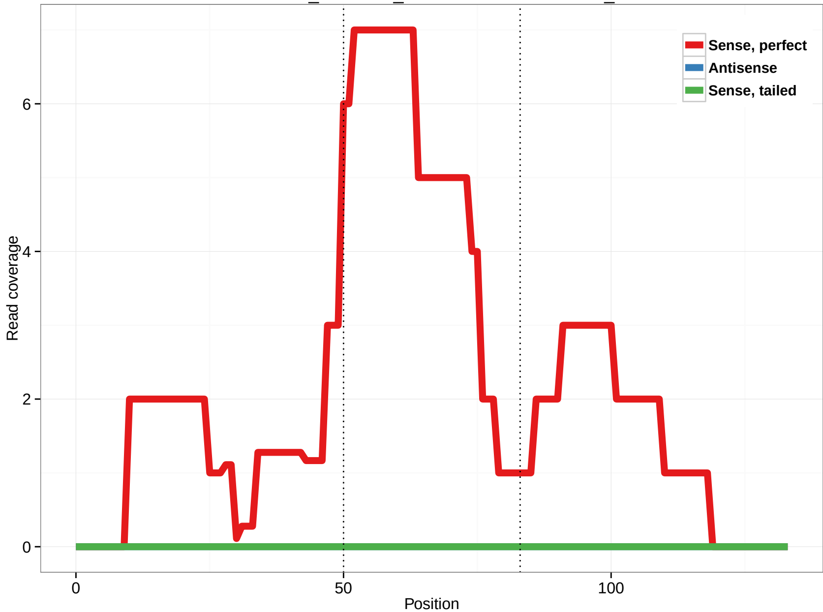
ornAna1_ensGene_ENSOANT00000015873_1
