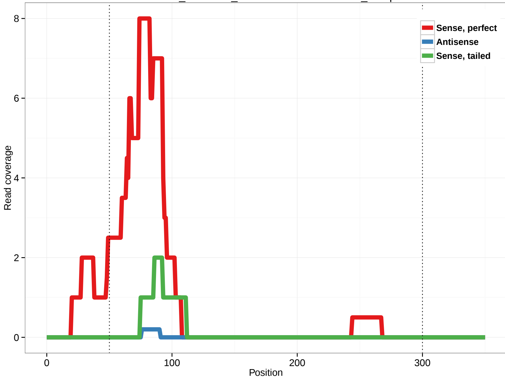
ornAna1_ensGene_ENSOANT00000015869_34.3p
