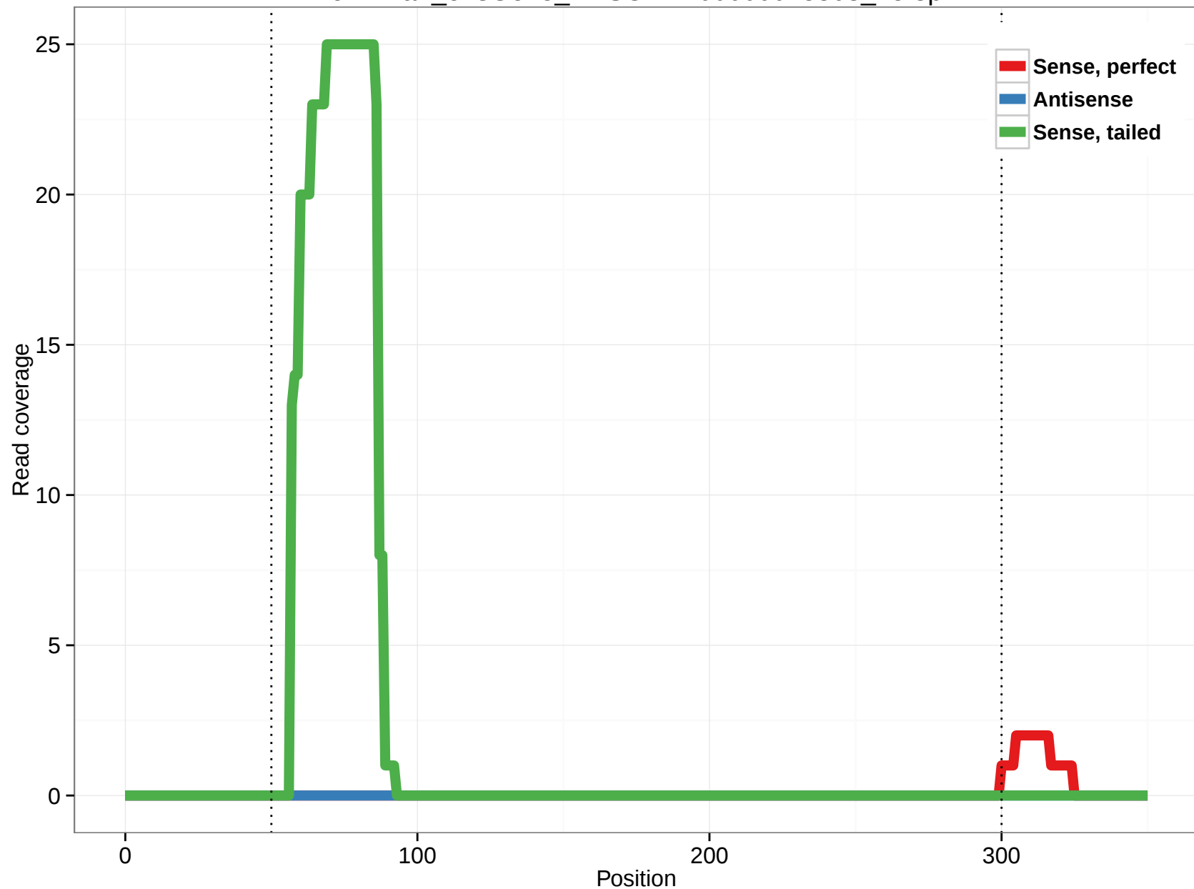
ornAna1_ensGene_ENSOANT00000015803_15.3p
