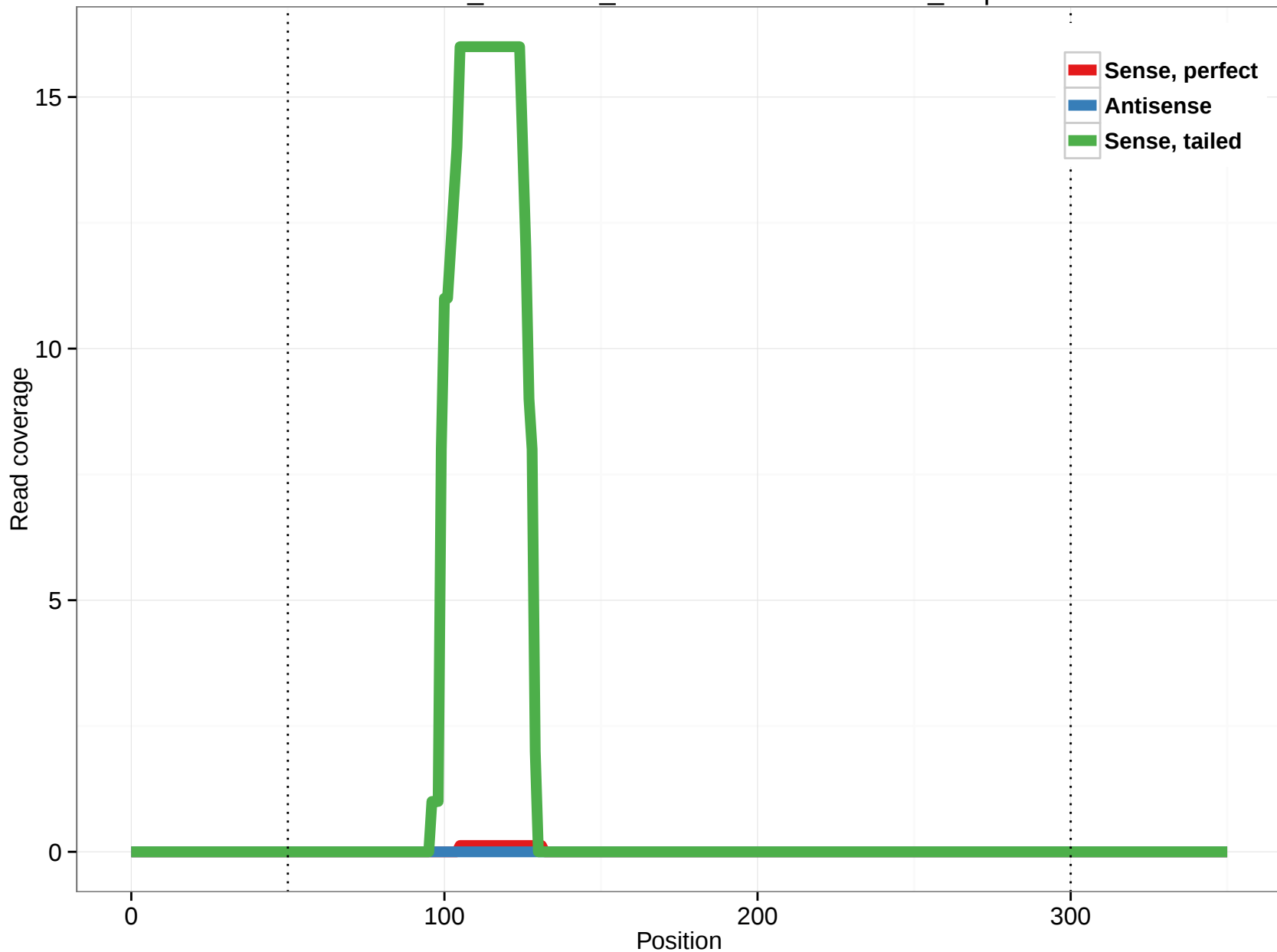
ornAna1_ensGene_ENSOANT00000015770_3.5p
