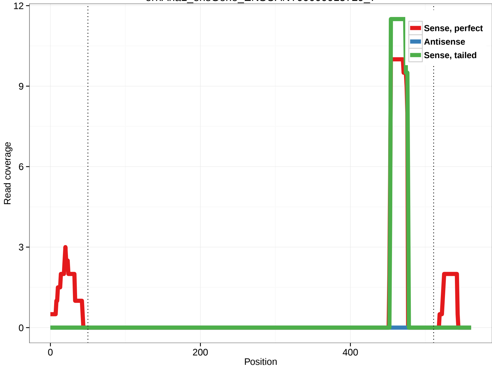
ornAna1_ensGene_ENSOANT00000015729_7
