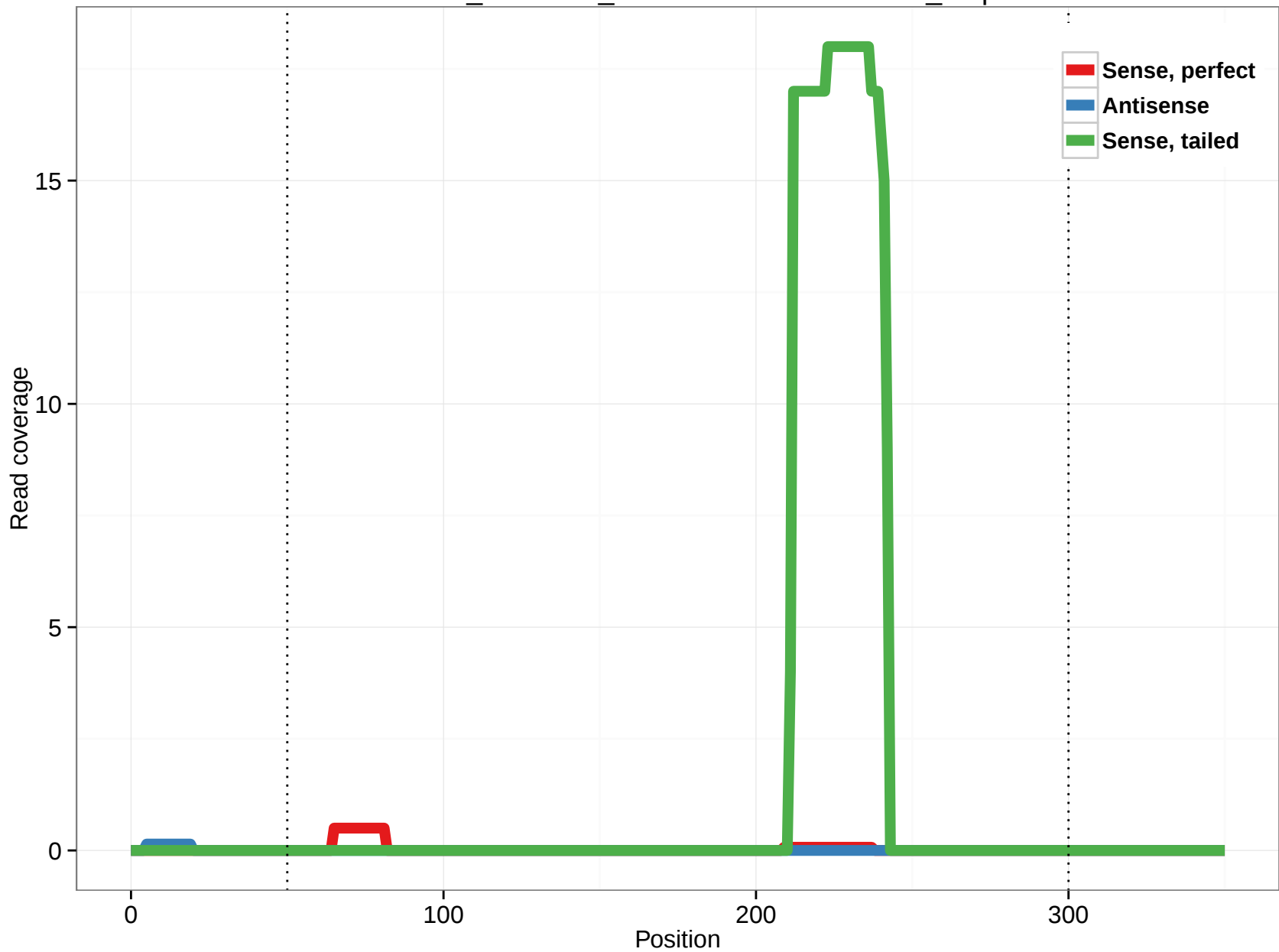
ornAna1_ensGene_ENSOANT00000015611_6.3p
