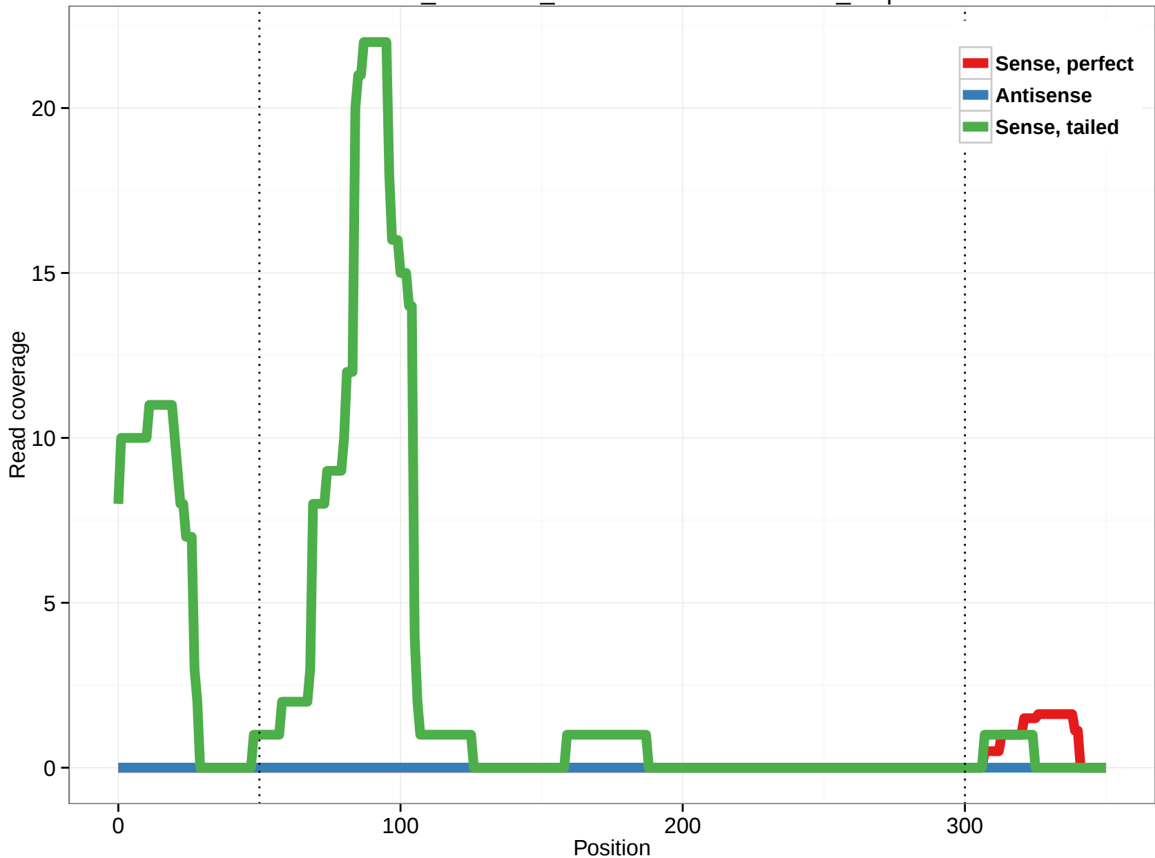
ornAna1_ensGene_ENSOANT00000015598_3.3p
