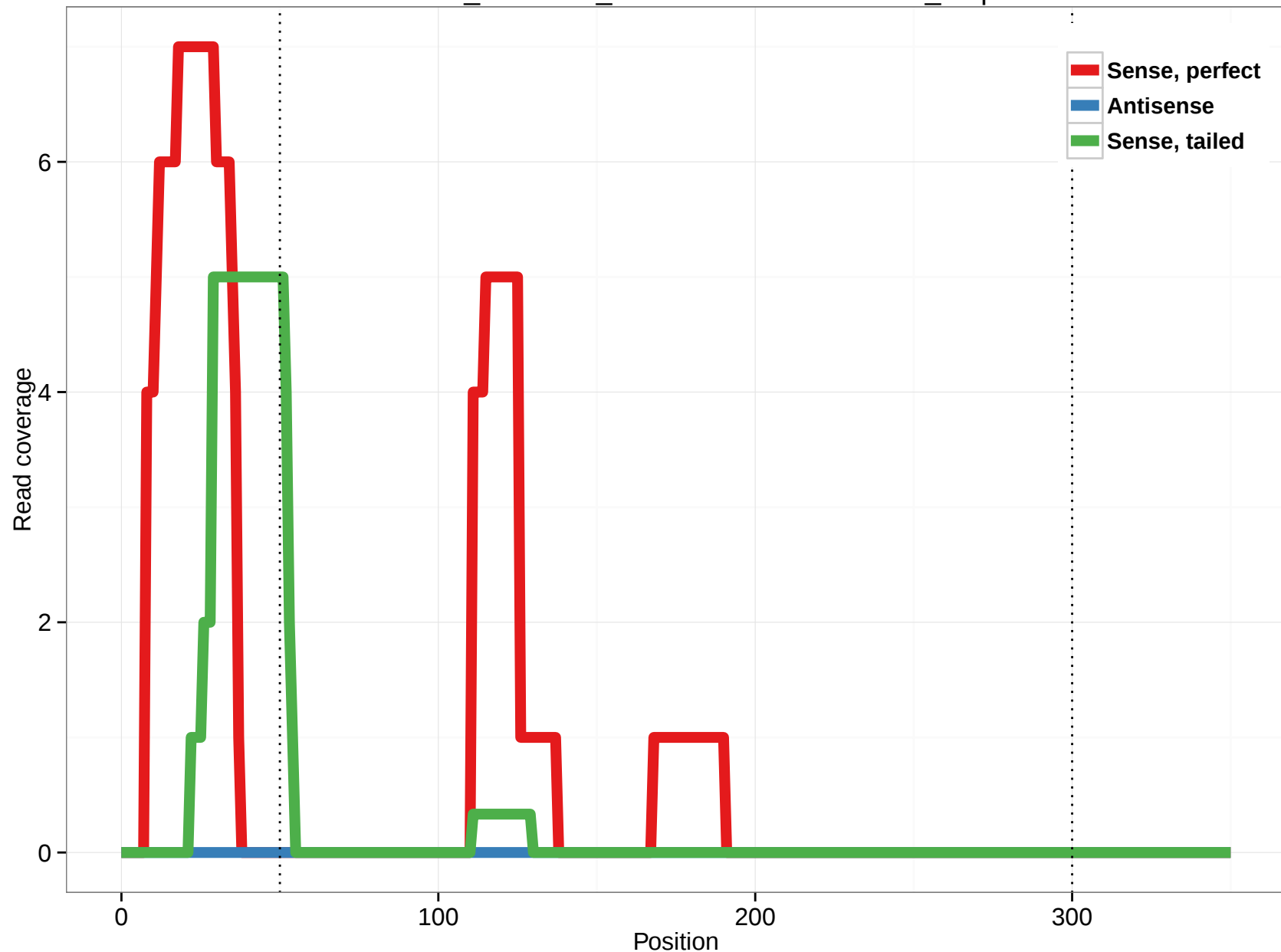
ornAna1_ensGene_ENSOANT00000015581_1.5p
