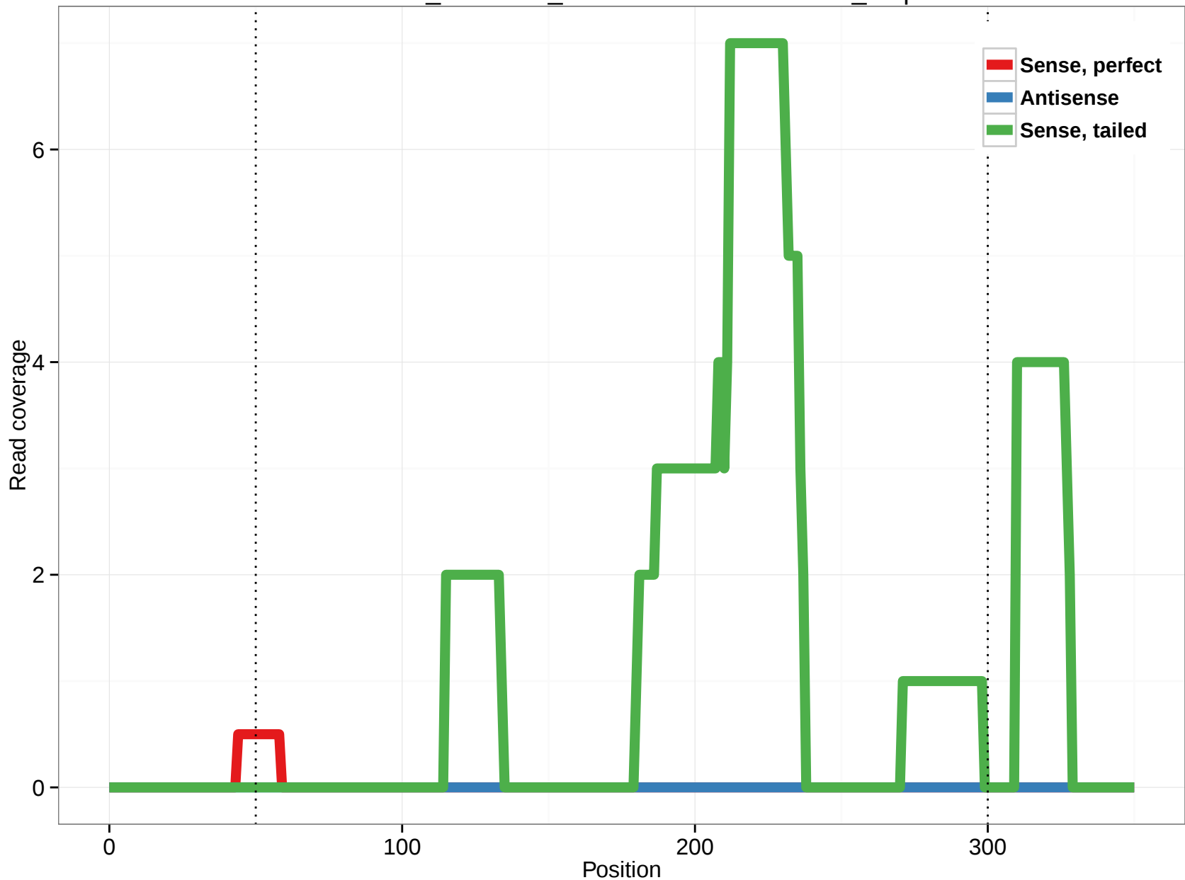
ornAna1_ensGene_ENSOANT00000015568_6.5p
