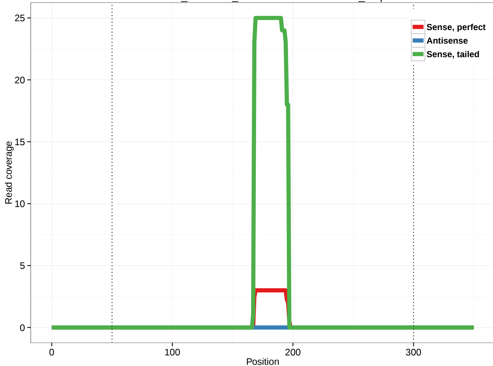
ornAna1_ensGene_ENSOANT00000015353_8.5p
