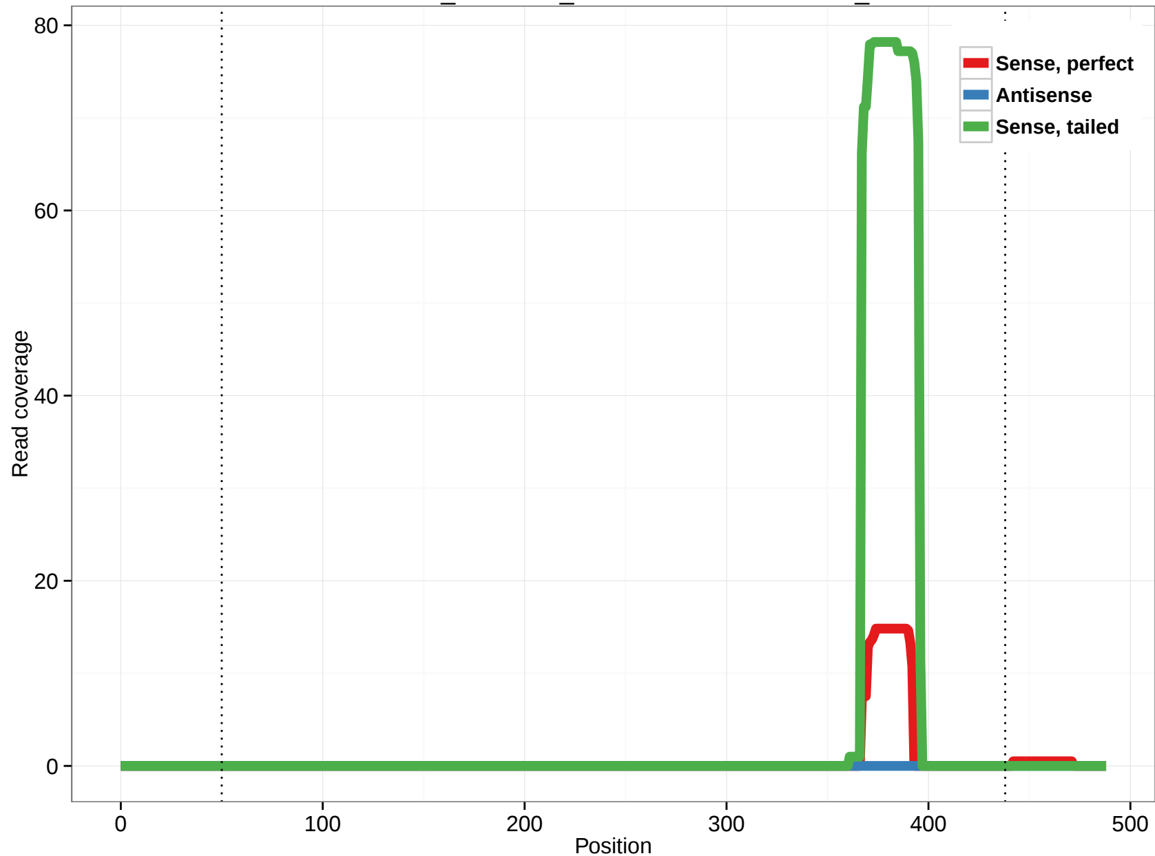
ornAna1_ensGene_ENSOANT00000015295_1
